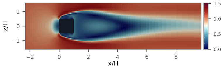
(a) |U|/U_b on the plane y/H = 0.5 at t^* = 80
