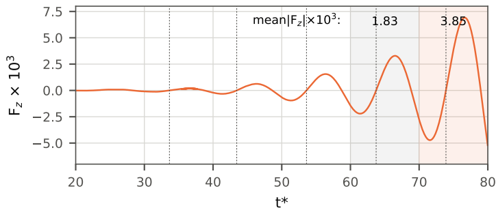
(c) Lateral force and complete-cycle boundaries
