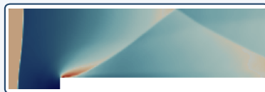
(b) Mach-2 step: Mach number, t = 4
