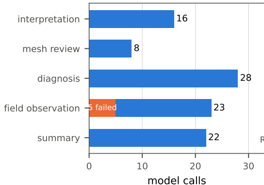
(a) 97 model calls in 19 sessions
