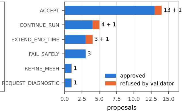
(b) 28 action proposals, 3 refused
