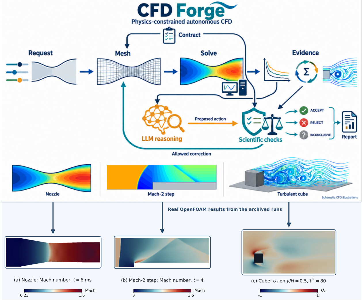
Figure 1: The CFD Forge workflow. Top: conceptual illustration (AI-generated, with the step tile redrawn by the authors; its flow pictures are schematic, not simulation output). A language model interprets the request and the simulation evidence and proposes actions; registered scientific checks, defined by each family’s contract, decide ACCEPT , REJECT , or INCONCLUSIVE and permit only listed corrections. Bottom: the corresponding real OpenFOAM fields from the archived runs, each with its own color scale. (a) Nozzle and (b) Mach-2 forward-facing step are from agent sessions; (c) the turbulent cube is a diagnostic study run outside the agent loop (Sec. 5.6).
