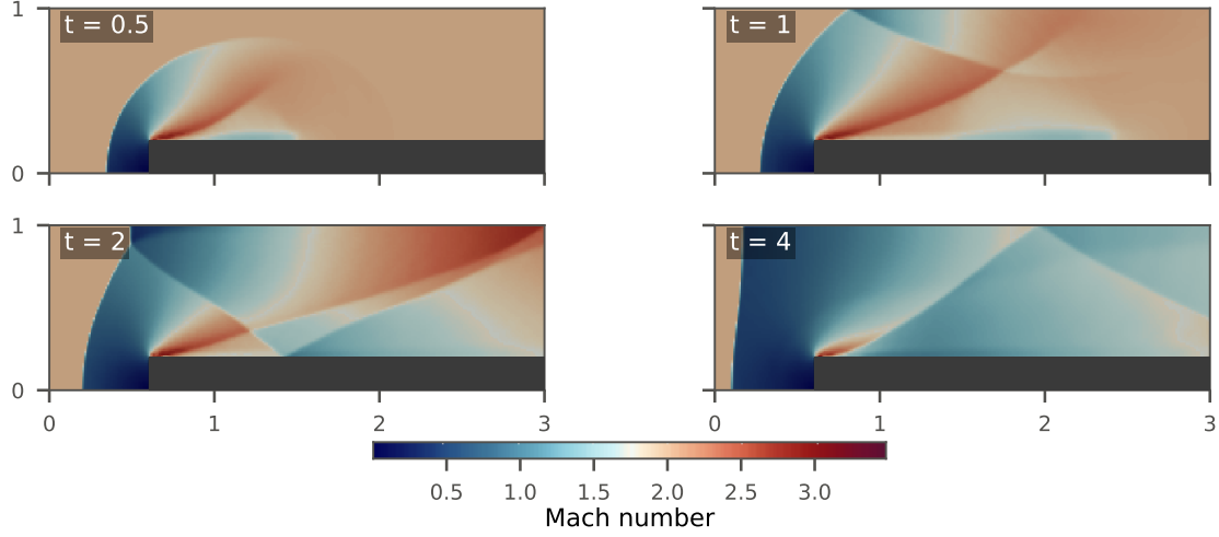
Figure 10: Evolution of the agent’s Mach-2 step solution: Mach number at t = 0.5, 1, 2, and 4 from the archived ParaView renderings of the native fields, on one fixed color range. The detached front moves upstream throughout, while the shoulder expansion and the reflected oblique shock reorganize behind it.
