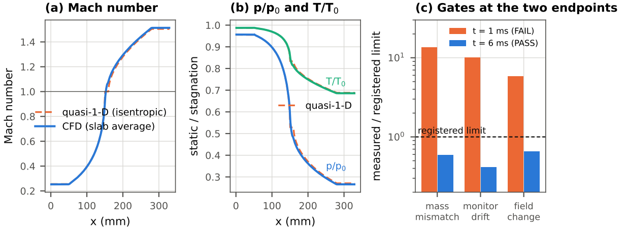
Figure 5: Nozzle results. (a,b) Axial profiles of the canonical run at t = 6 ms (solid) and the isentropic quasi-one-dimensional solution for the registered area distribution (dashed). (c) The three checks that failed at 1 ms in the separate continuation run (mass balance, monitor drift, field change), expressed as measured value over registered limit, at the initial 1 ms endpoint (failed) and after the approved continuation to 6 ms (passed).
