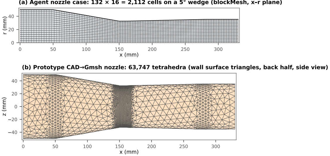
Figure 3: Nozzle meshes. (a) The agent-built wedge mesh in the x-r plane, every cell shown: five blocks with 20, 40, 4, 48, and 20 axial divisions and 16 radial divisions, reconstructed exactly from the archived blockMeshDict (linear edges, uniform grading), whose digest matches the native case. (b) The tetrahedral mesh from the earlier CAD→Gmsh prototype of the same nozzle (Appendix C): wall-surface triangles of the archived .msh file, back half only, viewed from the side, showing the throat refinement selected by the model.
