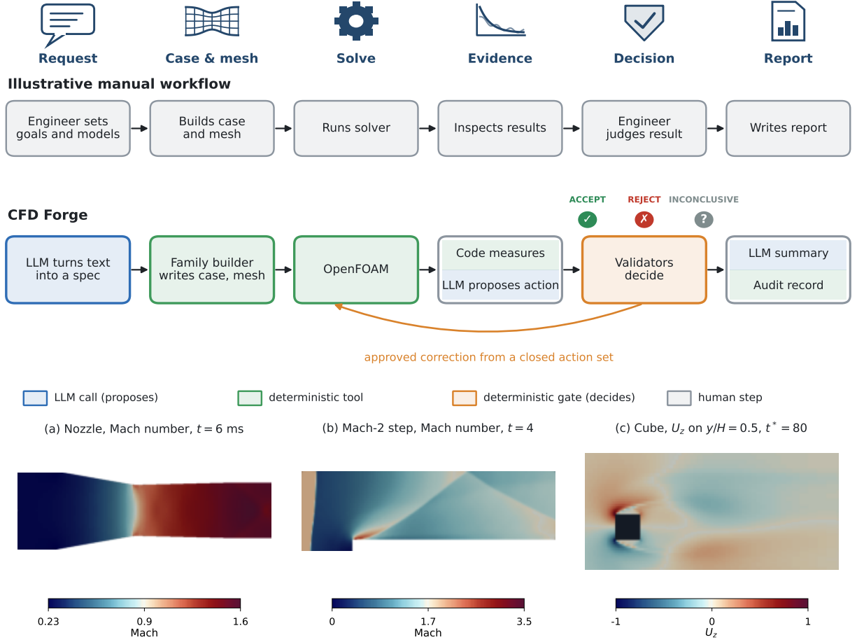
Figure 1: An illustrative manual CFD workflow (top) compared with CFD Forge (bottom). The manual row is a simplified illustration; conventional practice can also use scripted case construction and numerical diagnostics. Blue: language-model calls, which only propose; green: deterministic tools; orange: deterministic gates, which decide admissibility and acceptance; gray: human steps. Bottom: fields from the archived runs, each with its own color scale. (a) Nozzle and (b) Mach-2 forward-facing step are agent runs accepted under their family contracts; (c) the turbulent cube is a diagnostic study run outside the agent loop and not accepted (Sec. 5.6).
