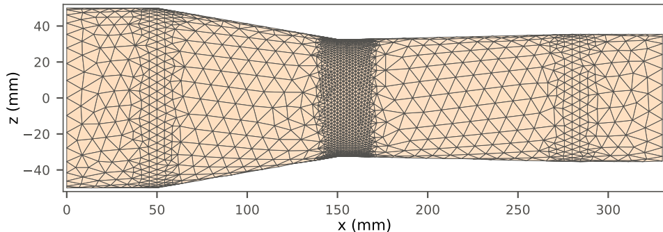
(b) Prototype CAD→Gmsh nozzle: 63,747 tetrahedra (wall surface triangles, back half, side view)
