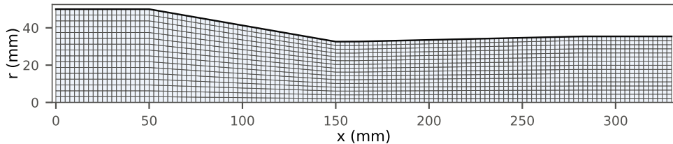
(a) Agent nozzle case: 132 \times 16 = 2,112 cells on a 5^\circ wedge (blockMesh, x-r plane)
