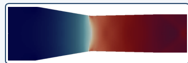
(a) Nozzle: Mach number, t = 6 ms
