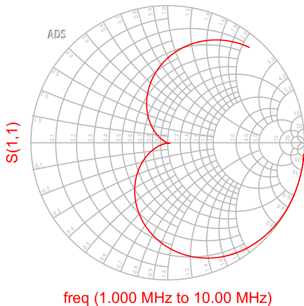
Input Reflection Coefficient
