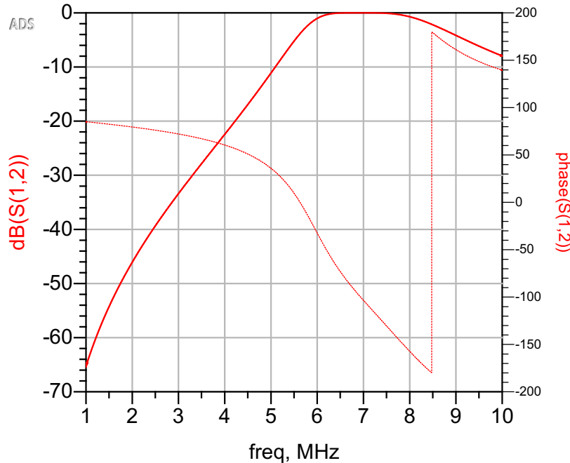
Reverse Transmission, dB
