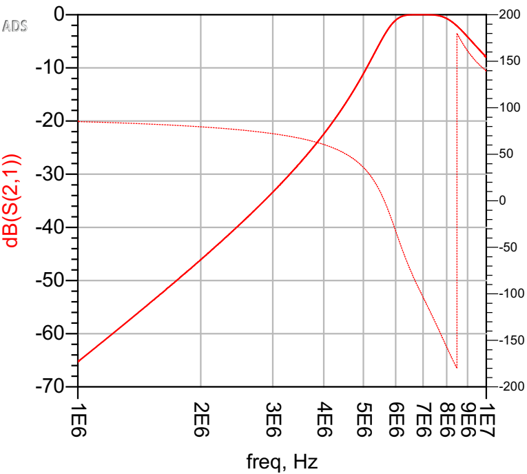
Forward Transmission, dB
