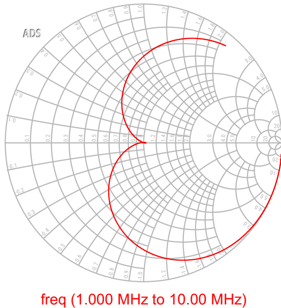
Output Reflection Coefficient
