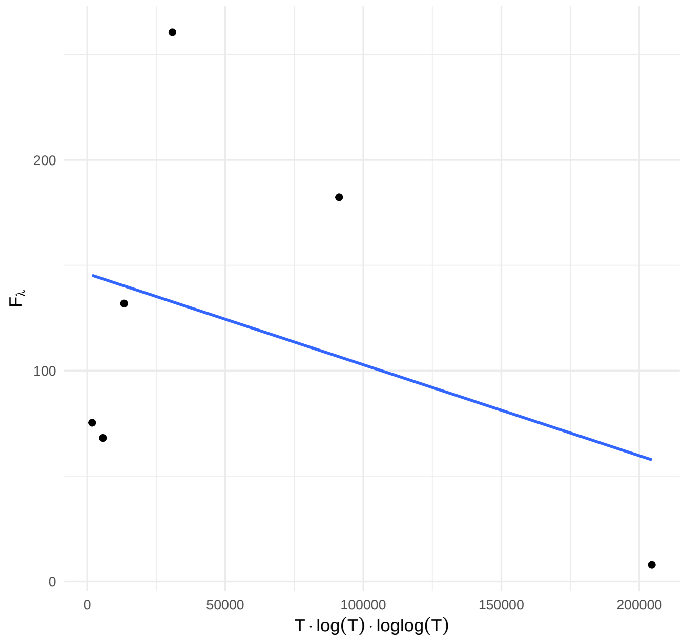
F_\lambda vs T \times \log(T) \times \log\log(T)
