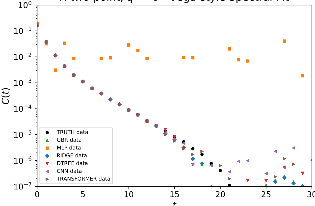
K two-point, q^2 = 0 - Vega-style Spectral Fit
