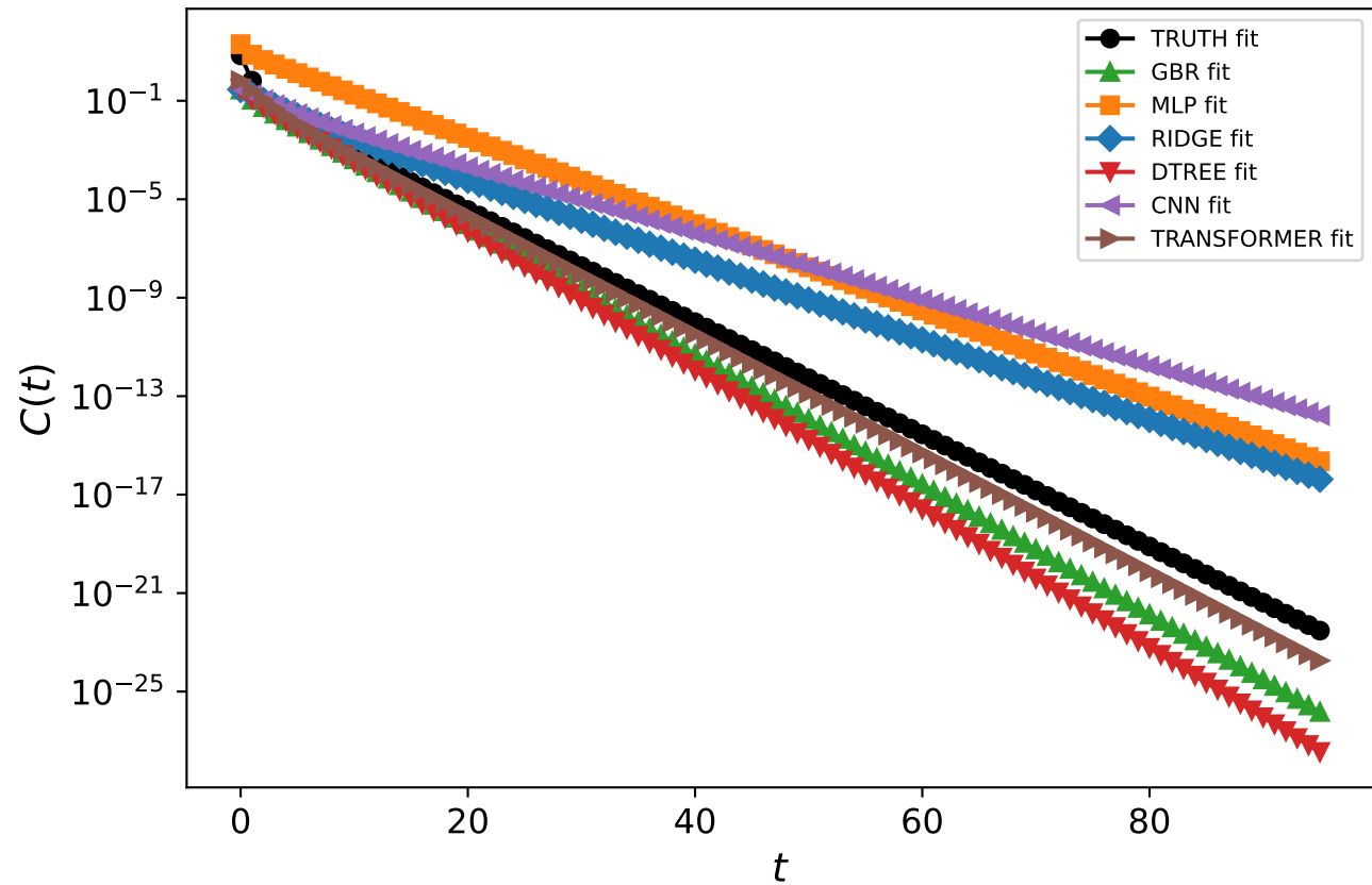
K two-point, q^2 = 0 - Simple Spectral Fit
