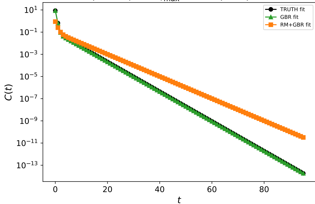
K two-point, q^2 = 2q_{\text{max}}^2/3 - Simple Spectral Fit
