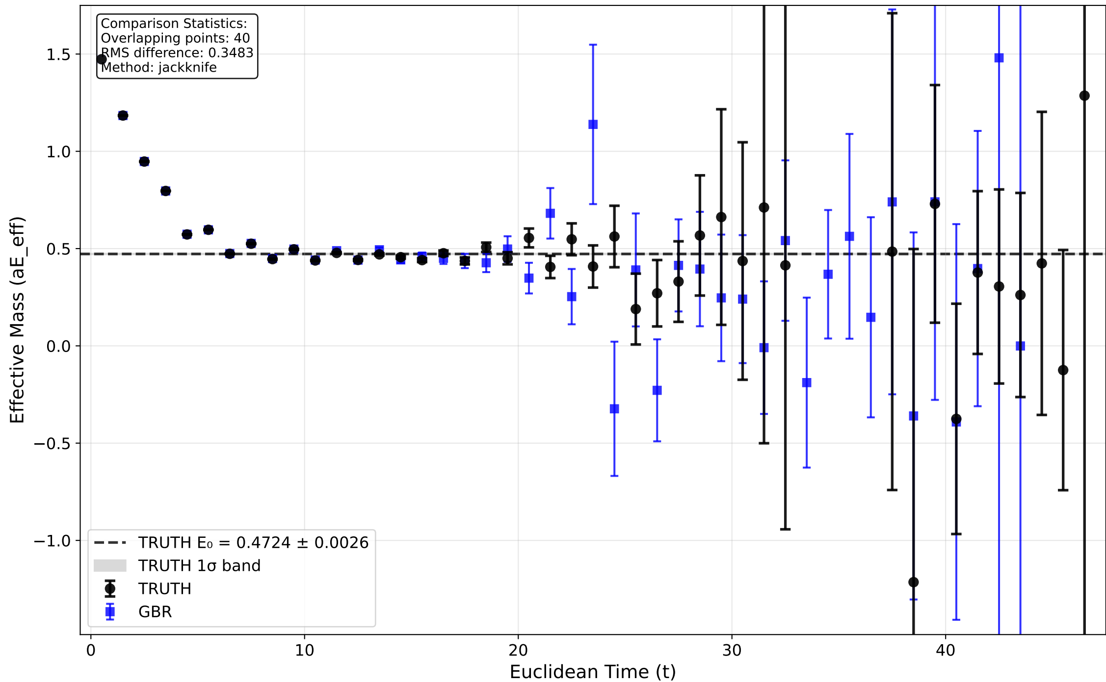
Effective Mass Comparison: TRUTH vs GBR
