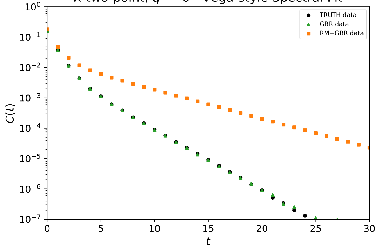
K two-point, q^2 = 0 - Vega-style Spectral Fit
