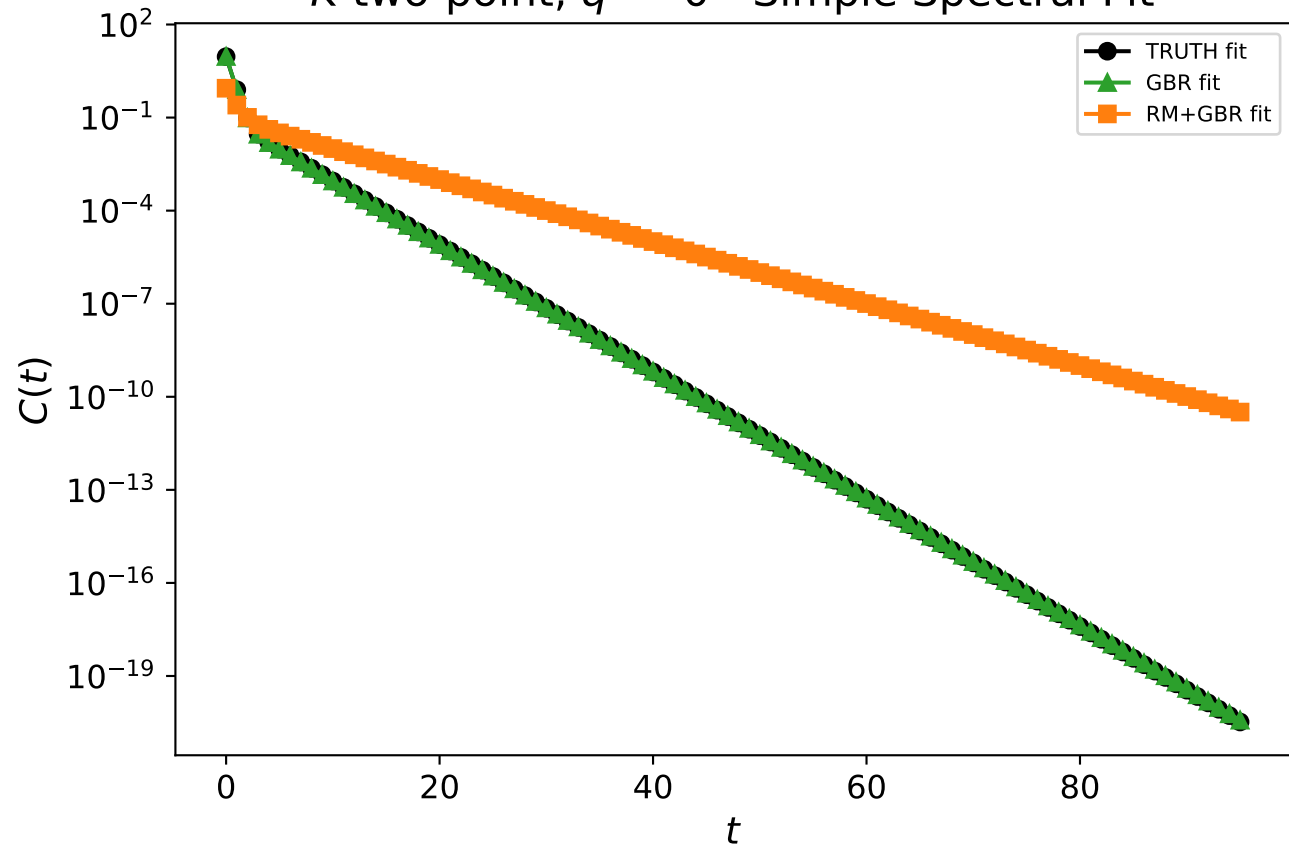
K two-point, q^2 = 0 - Simple Spectral Fit
