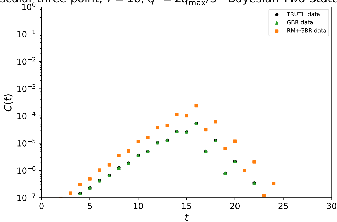
Local scalar three-point, T = 16 , q^2 = 2q_{\text{max}}^2/3 - Bayesian Two-State Spectral Fit
