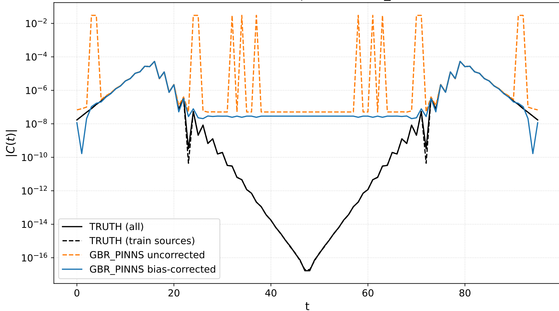
Full correlator comparison (GBR_PINNS)
