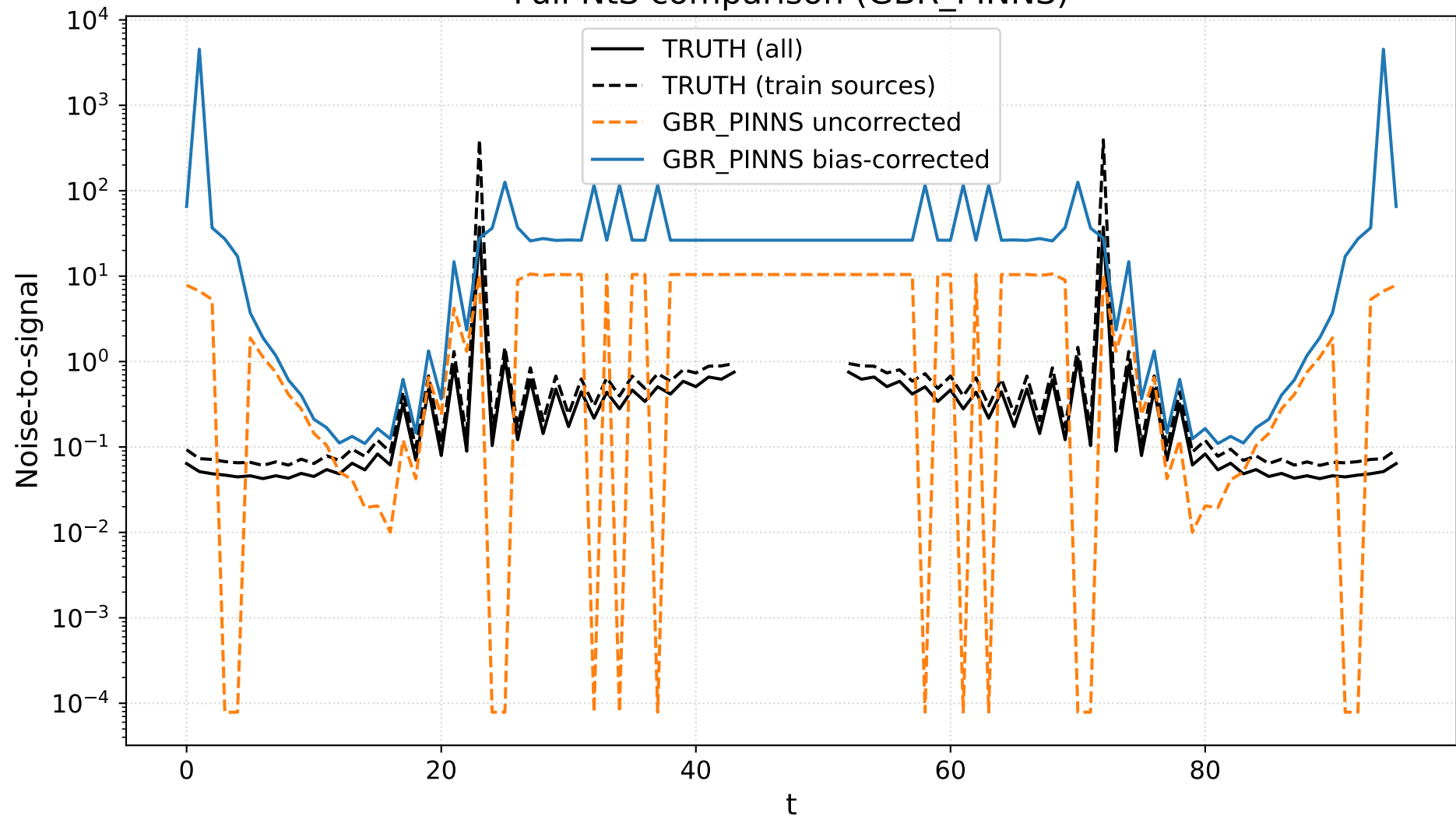
Full NtS comparison (GBR_PINNS)
