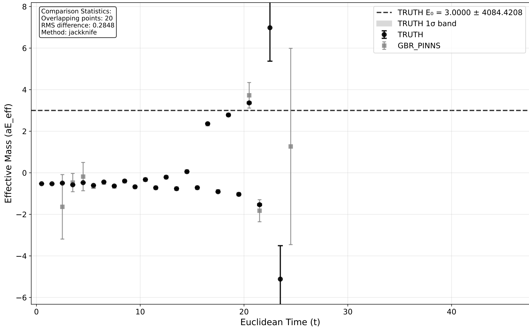
Effective Mass Comparison: TRUTH vs GBR_PINNS
