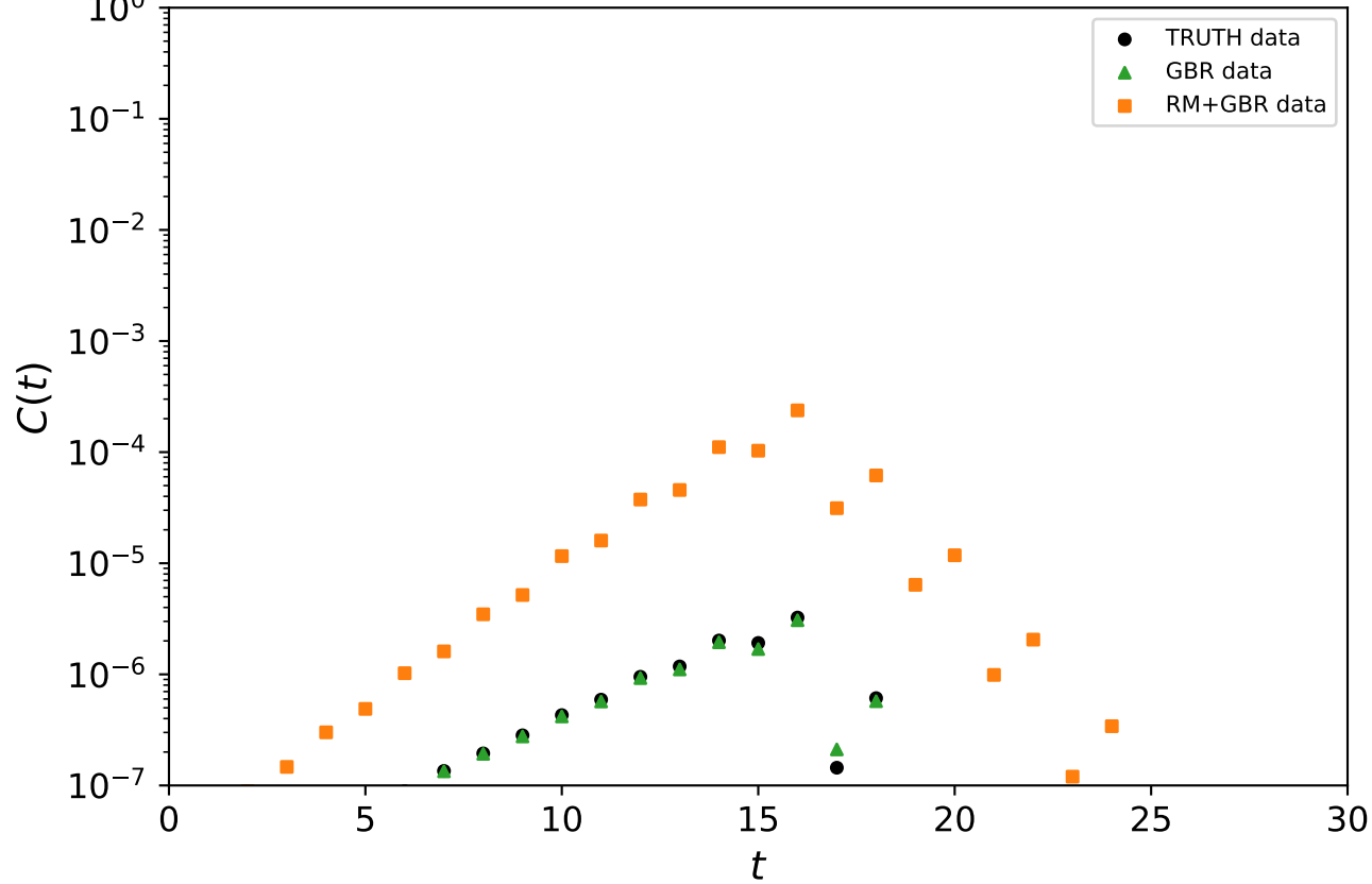
Local scalar three-point, T = 16 , q^2 = 0 - Bayesian Two-State Spectral Fit
