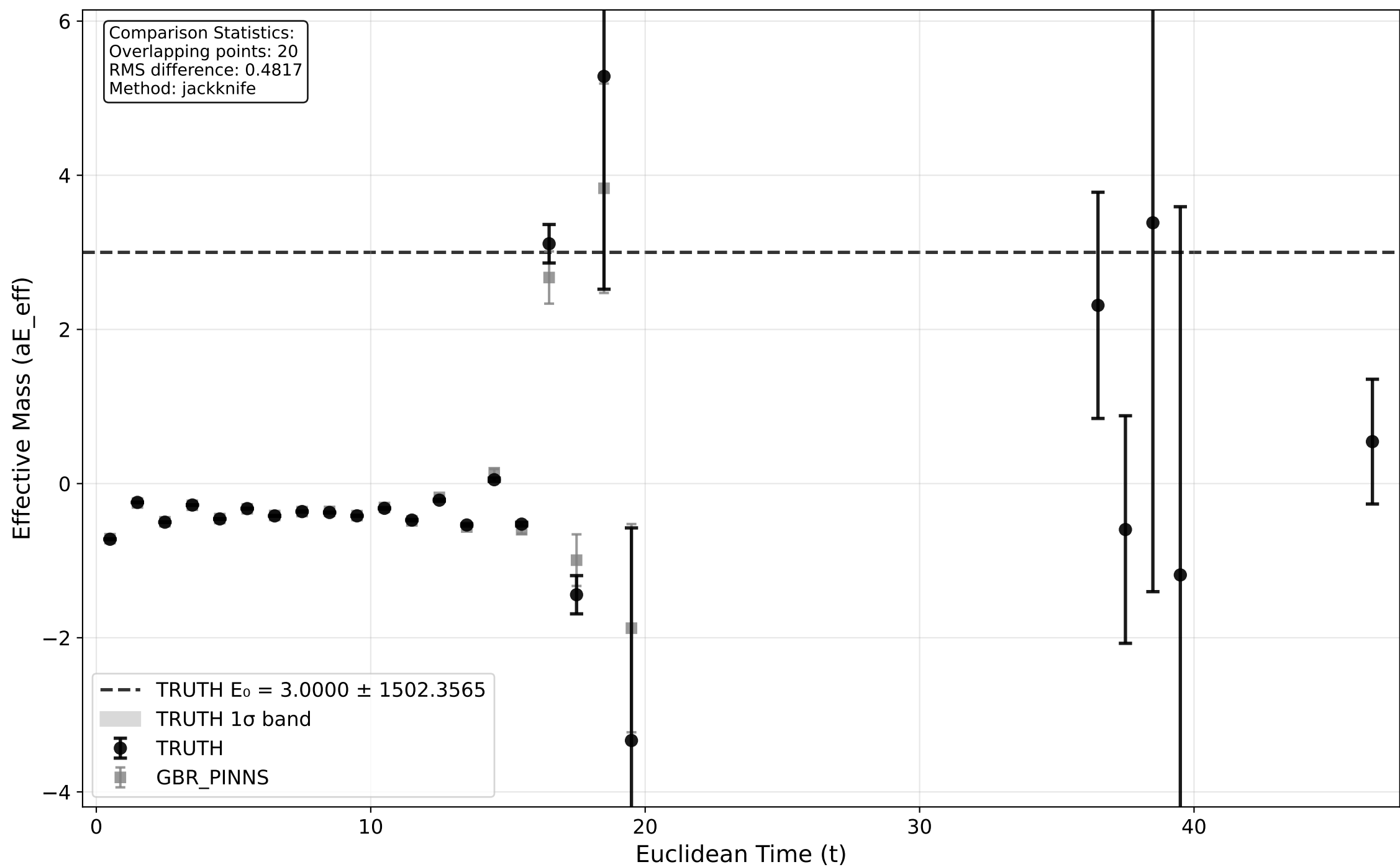
Effective Mass Comparison: TRUTH vs GBR_PINNS
