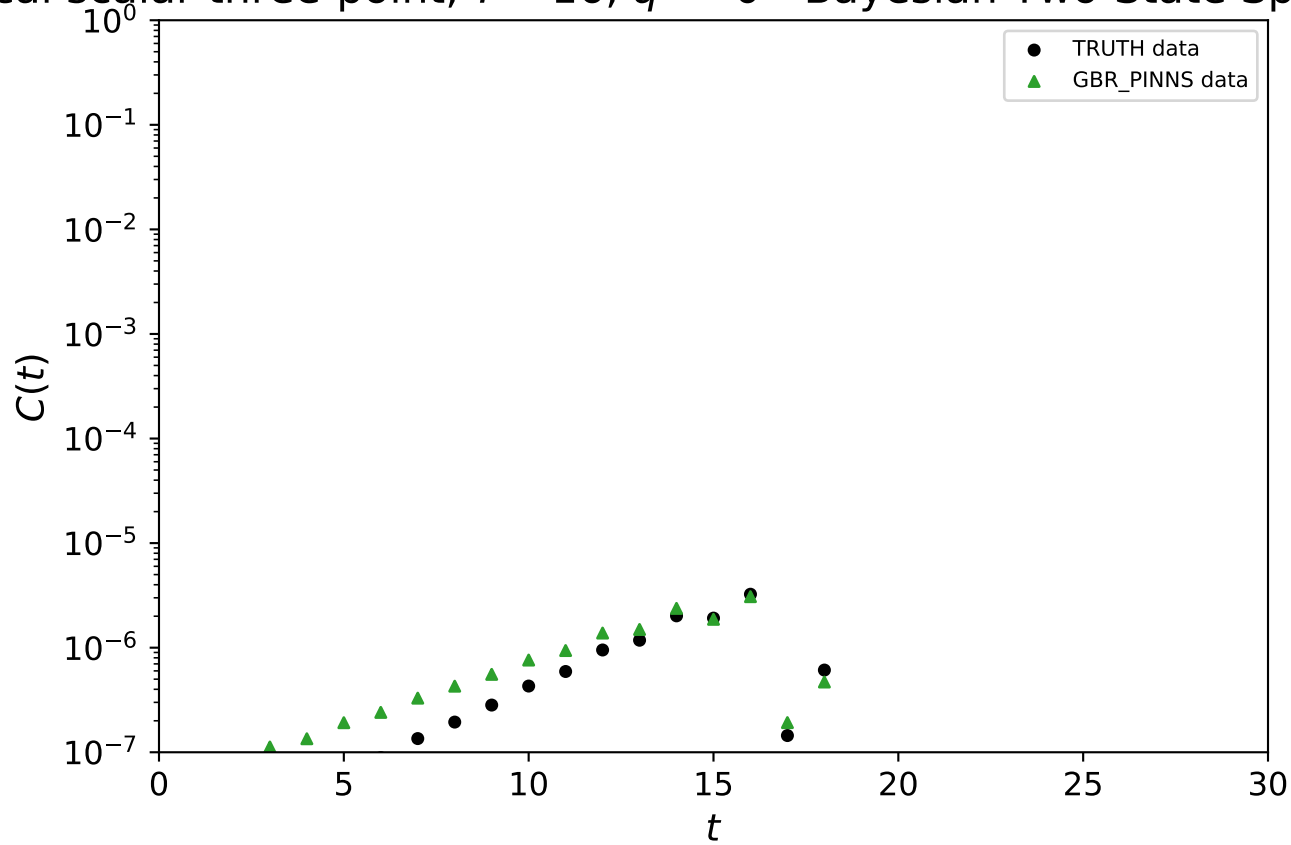
Local scalar three-point, T = 16 , q^2 = 0 - Bayesian Two-State Spectral Fit
