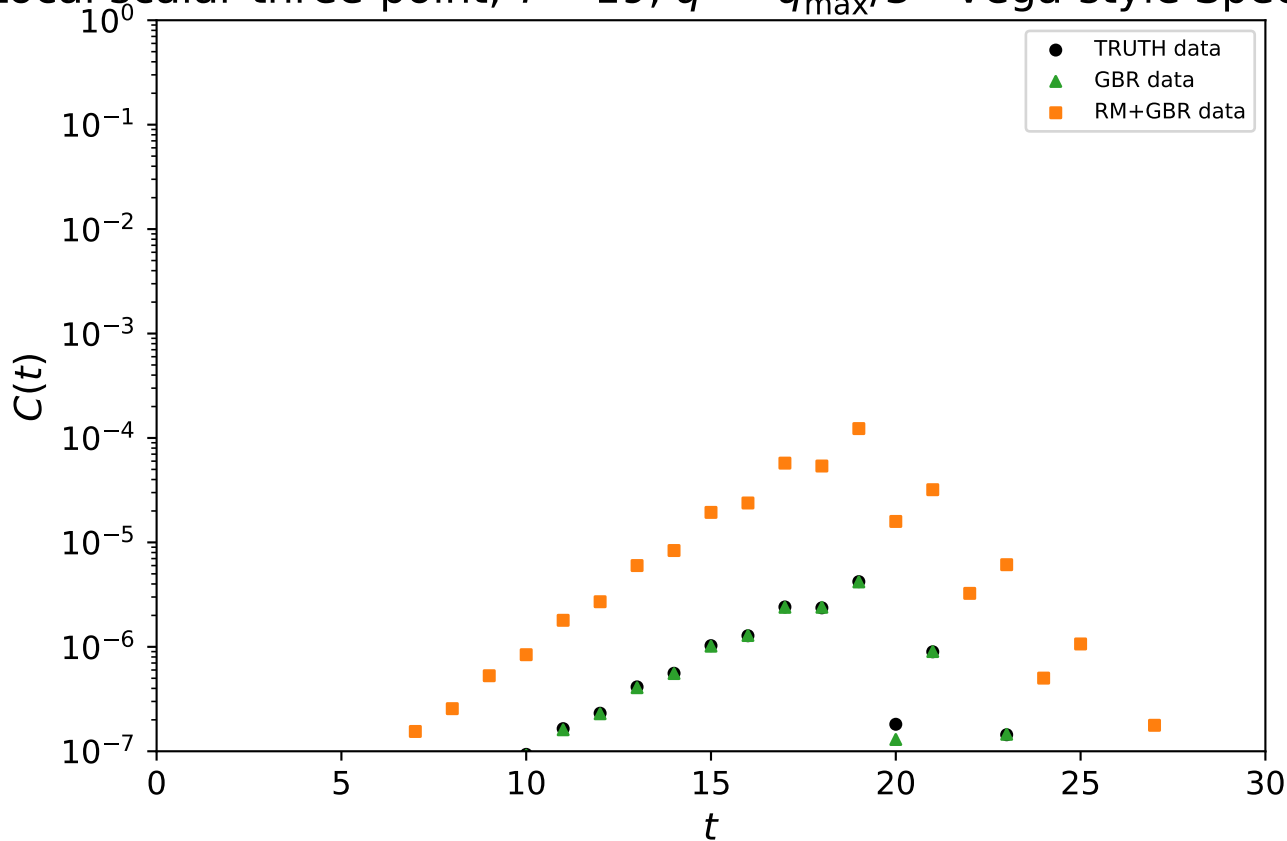
Local scalar three-point, T = 19 , q^2 = q_{\text{max}}^2/3 - Vega-style Spectral Fit
