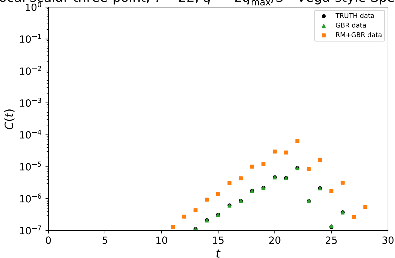
Local scalar three-point, T = 22 , q^2 = 2q_{\text{max}}^2/3 - Vega-style Spectral Fit
