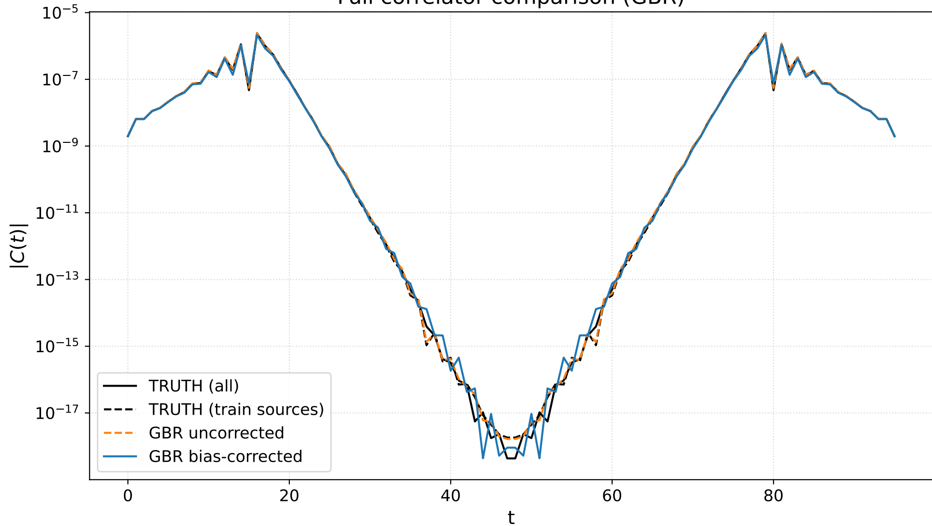
Full correlator comparison (GBR)
