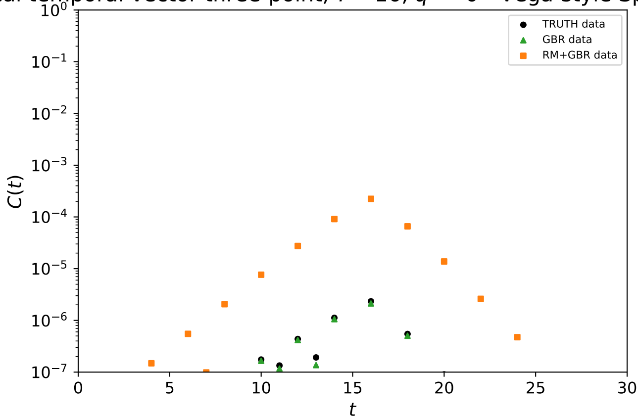
Local temporal vector three-point, T = 16 , q^2 = 0 - Vega-style Spectral Fit
