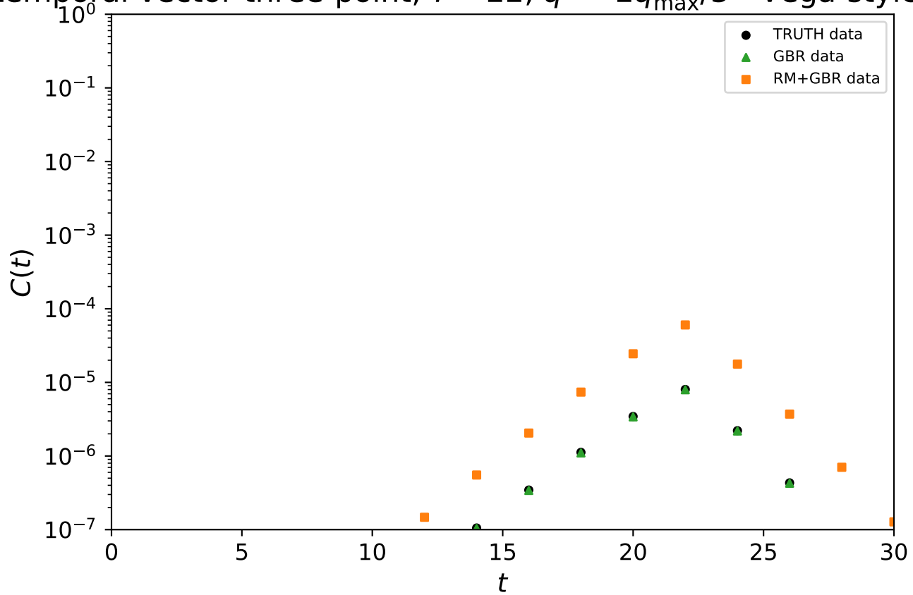
Local temporal vector three-point, T = 22 , q^2 = 2q_{\text{max}}^2/3 - Vega-style Spectral Fit
