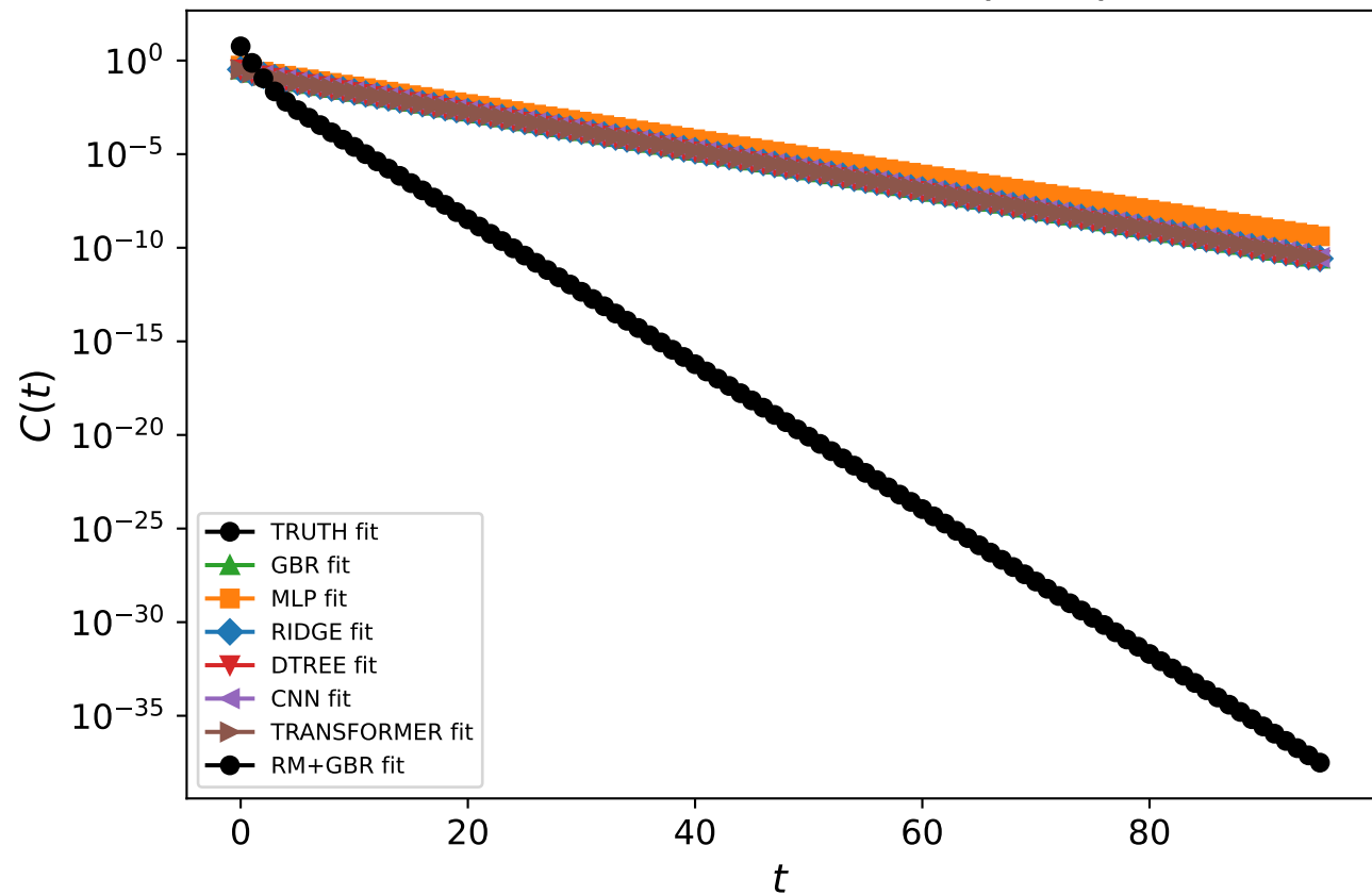
D meson, Gold to non-Gold - Simple Spectral Fit
