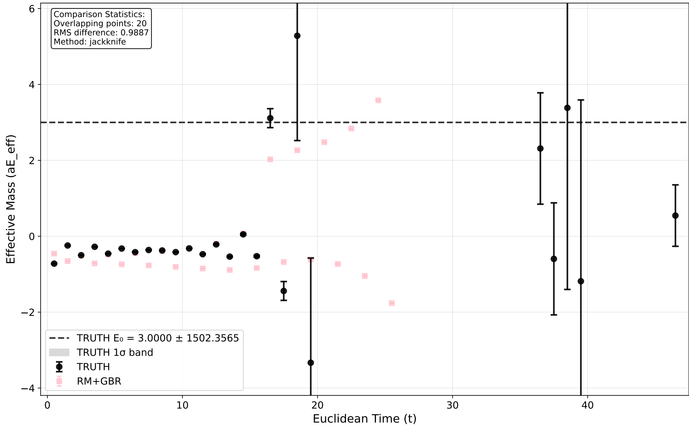
Effective Mass Comparison: TRUTH vs RM+GBR
