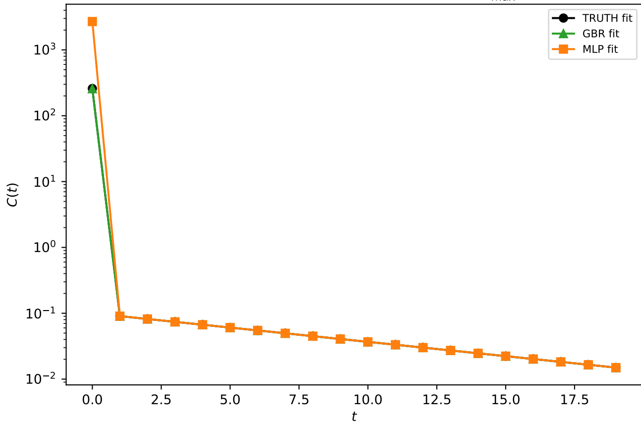
Local scalar three-point, T = 19 , q^2 = 2q_{\text{max}}^2/3
