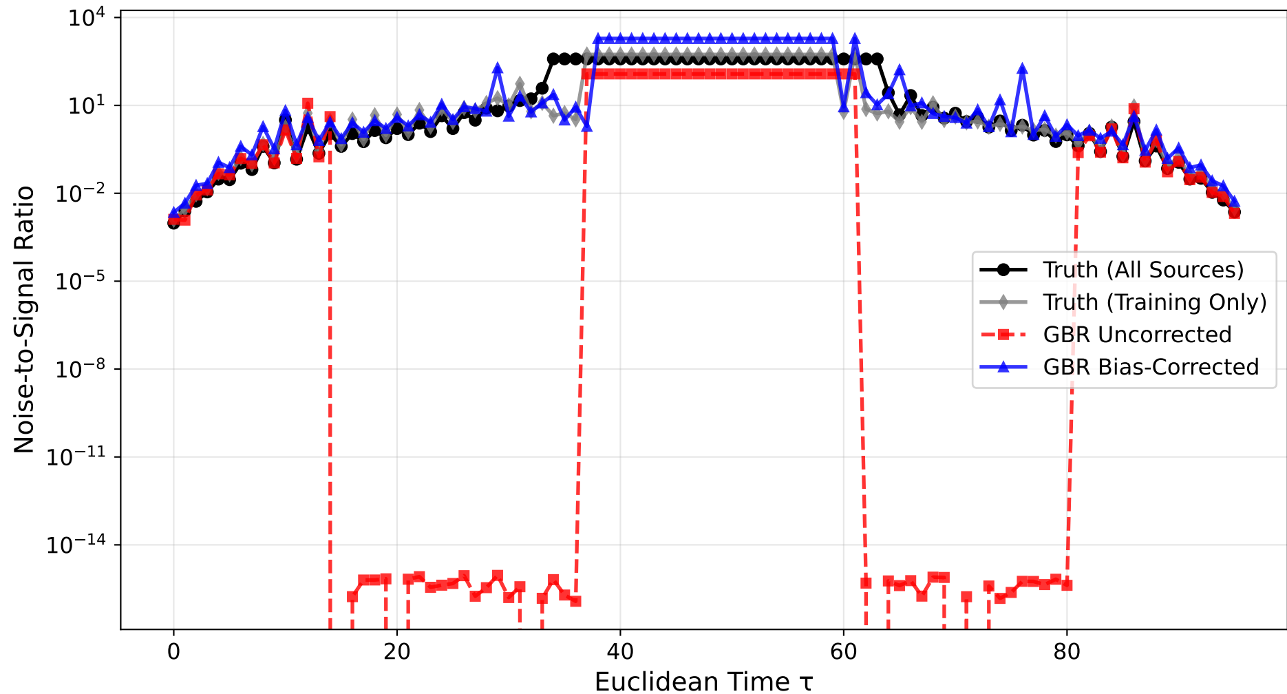
NtS Comparison - GBR
