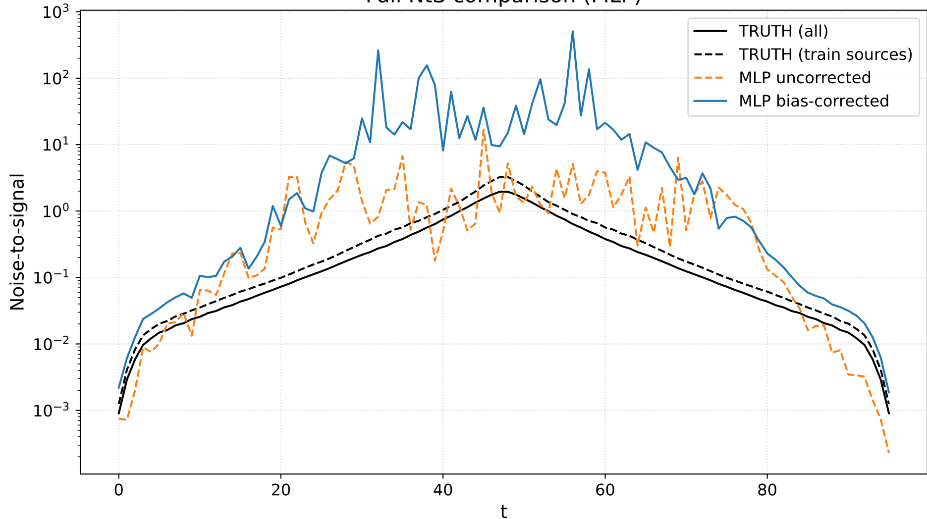
Full NtS comparison (MLP)
