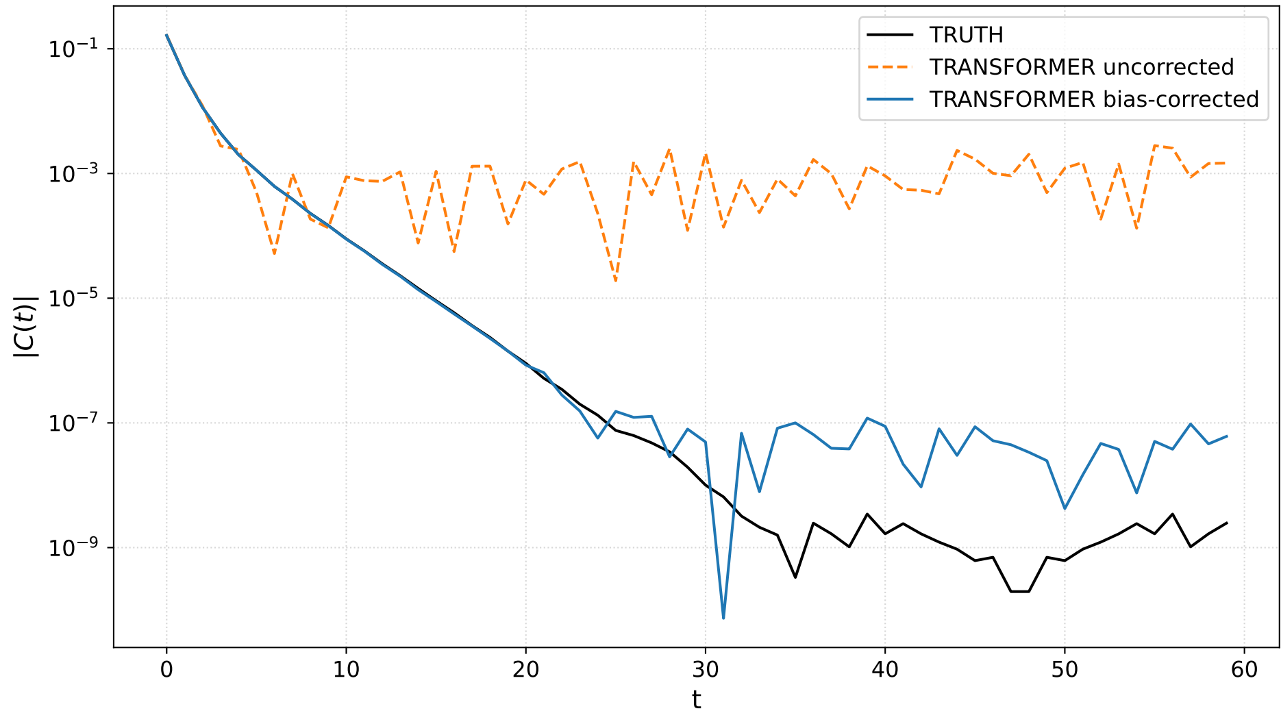
Bias correction effect (TRANSFORMER)
