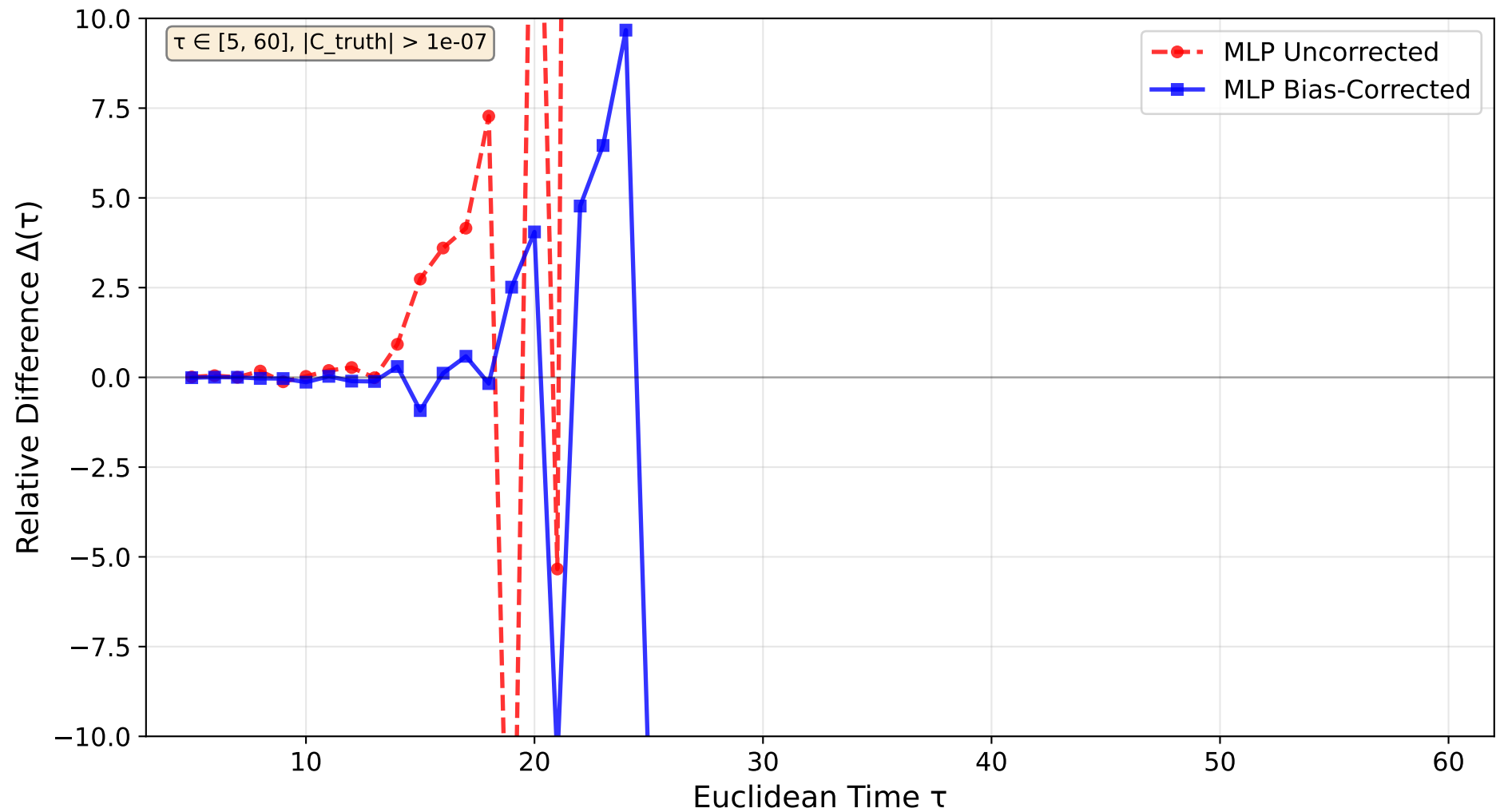
Bias Correction Effect - MLP
