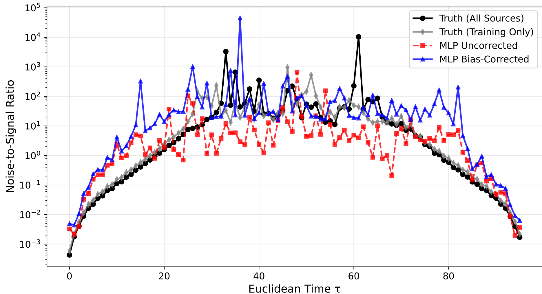
NtS Comparison - MLP
