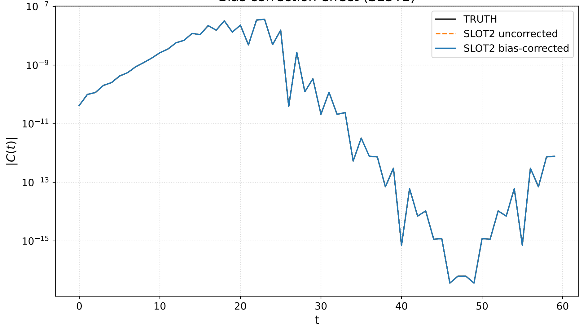
Bias correction effect (SLOT2)
