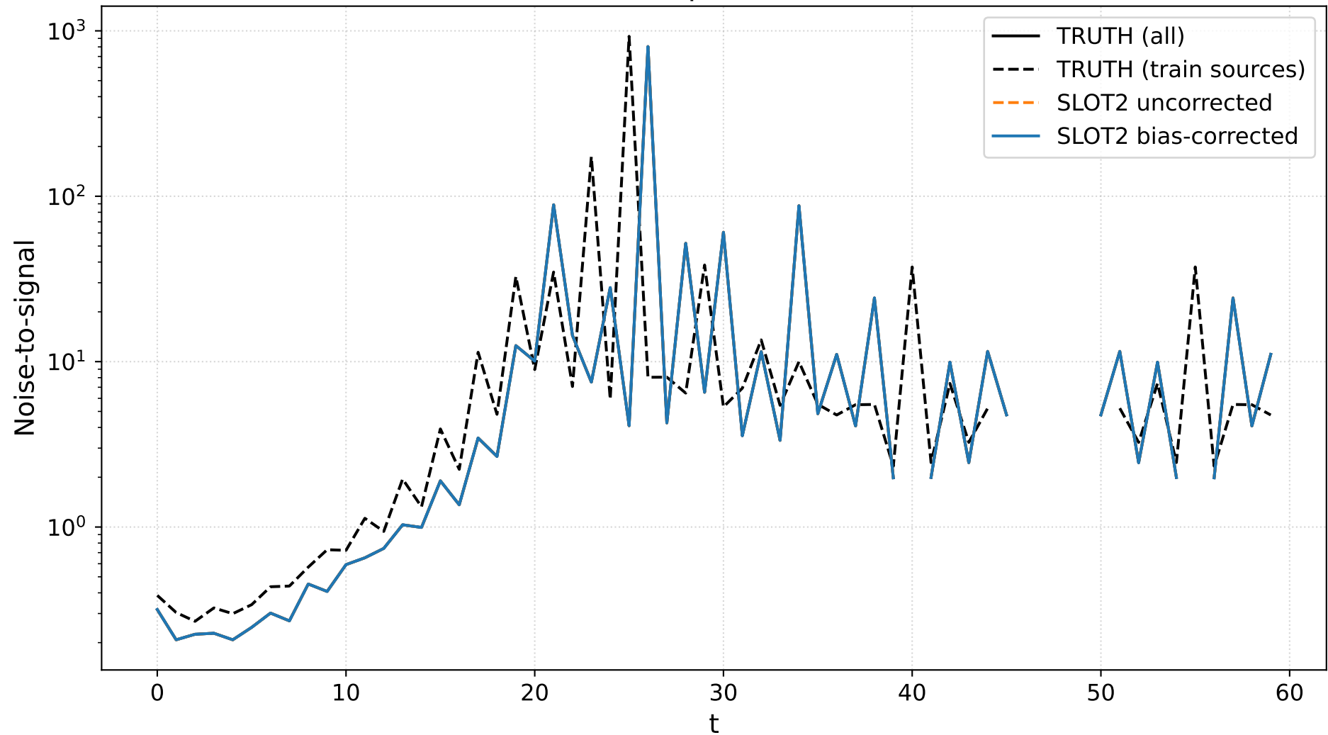
Full NtS comparison (SLOT2)
