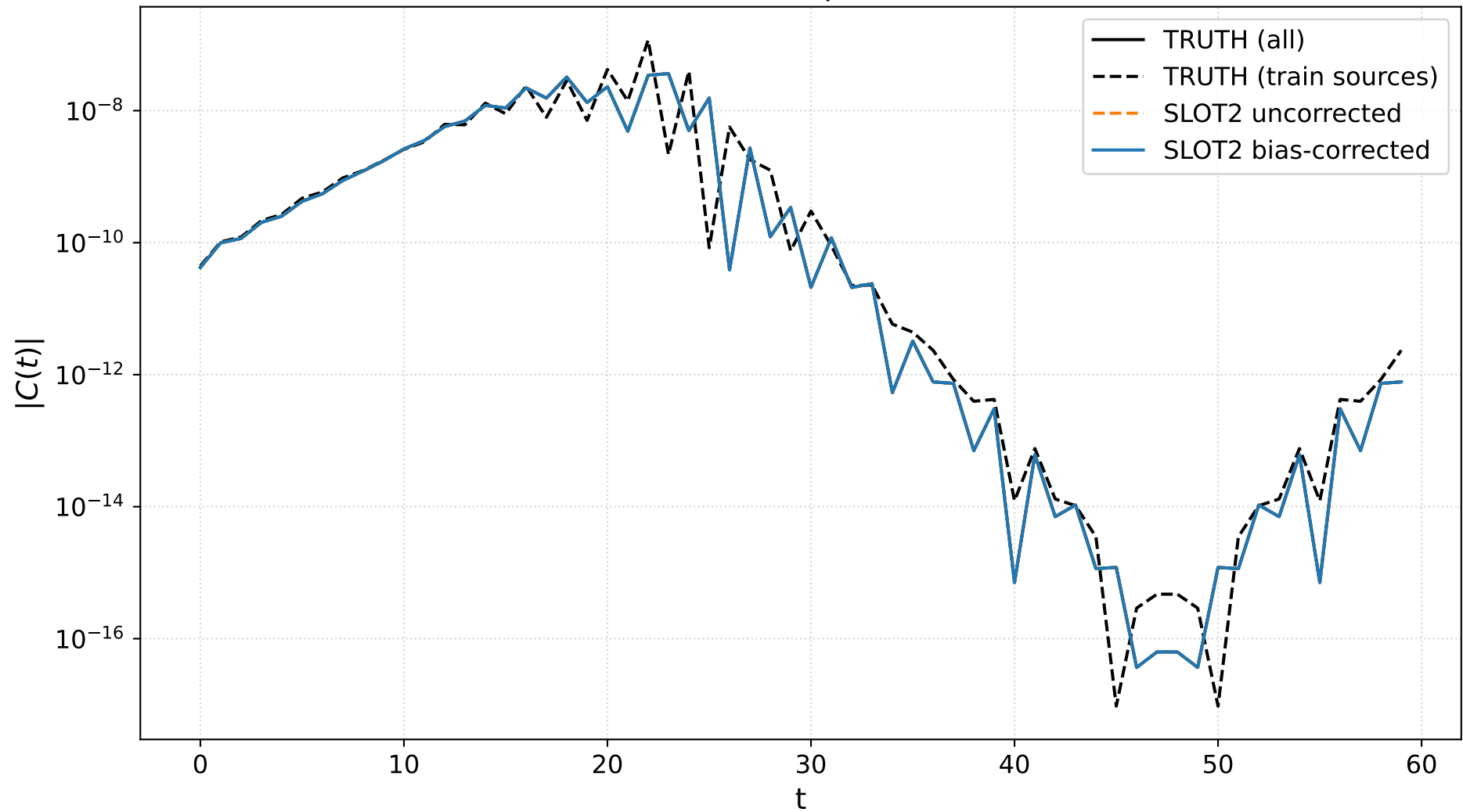
Full correlator comparison (SLOT2)
