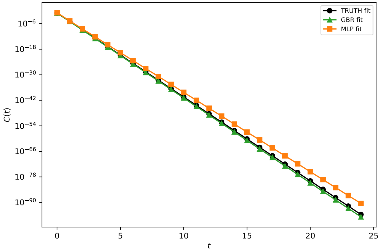
K two-point, q^2 = 0
