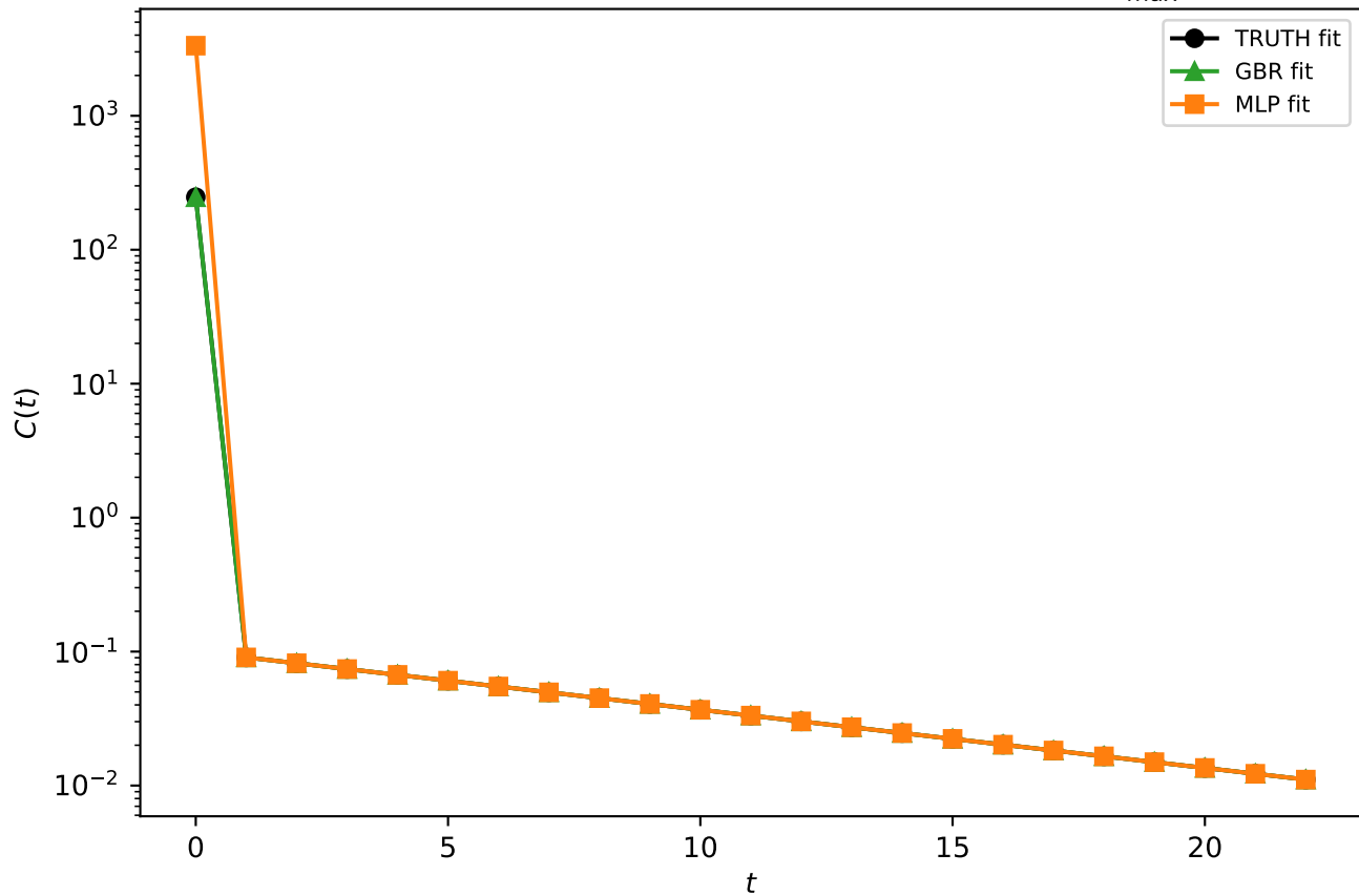
Local temporal vector three-point, T = 22 , q^2 = 2q_{\max}^2/3
