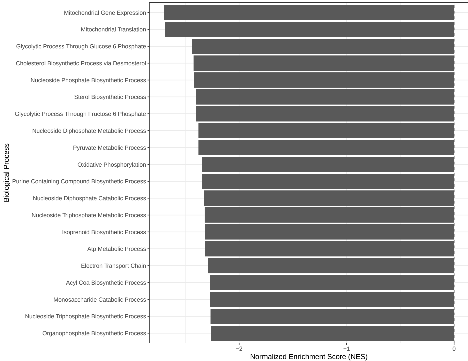
GSE168404 PCOS: Top GO Biological Processes
