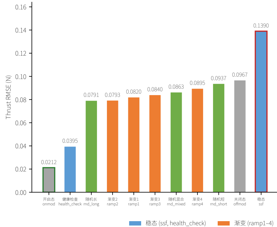
Thrust RMSE by Operating Mode
