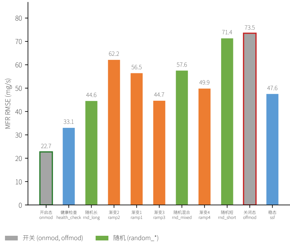
MFR RMSE by Operating Mode
