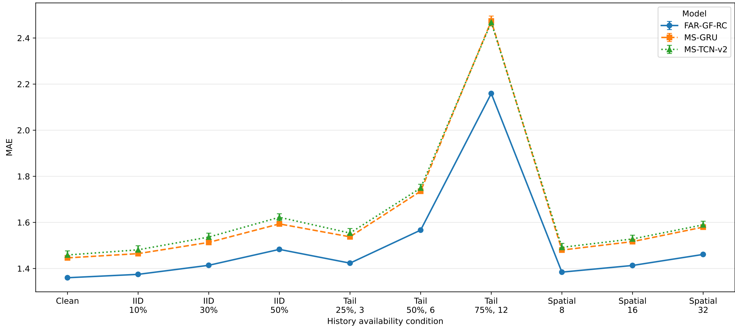
Horizon 3 forecasting MAE under controlled sensor dropout
