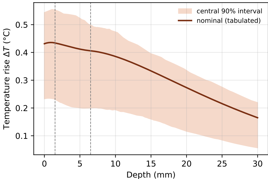
Steady-state \Delta T vs depth, 2.45 GHz, 50 W/m 2
