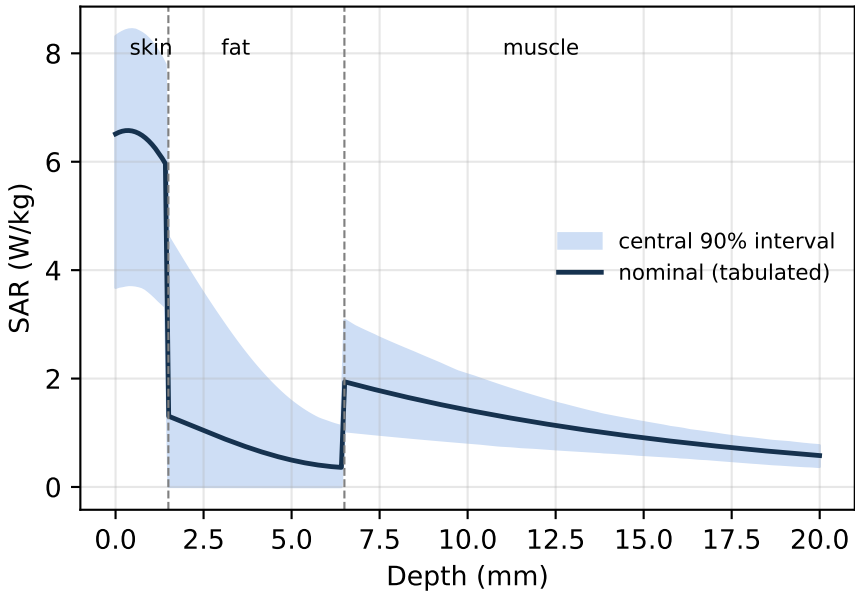
Local SAR vs depth, 2.45 GHz, 50 W/m 2
