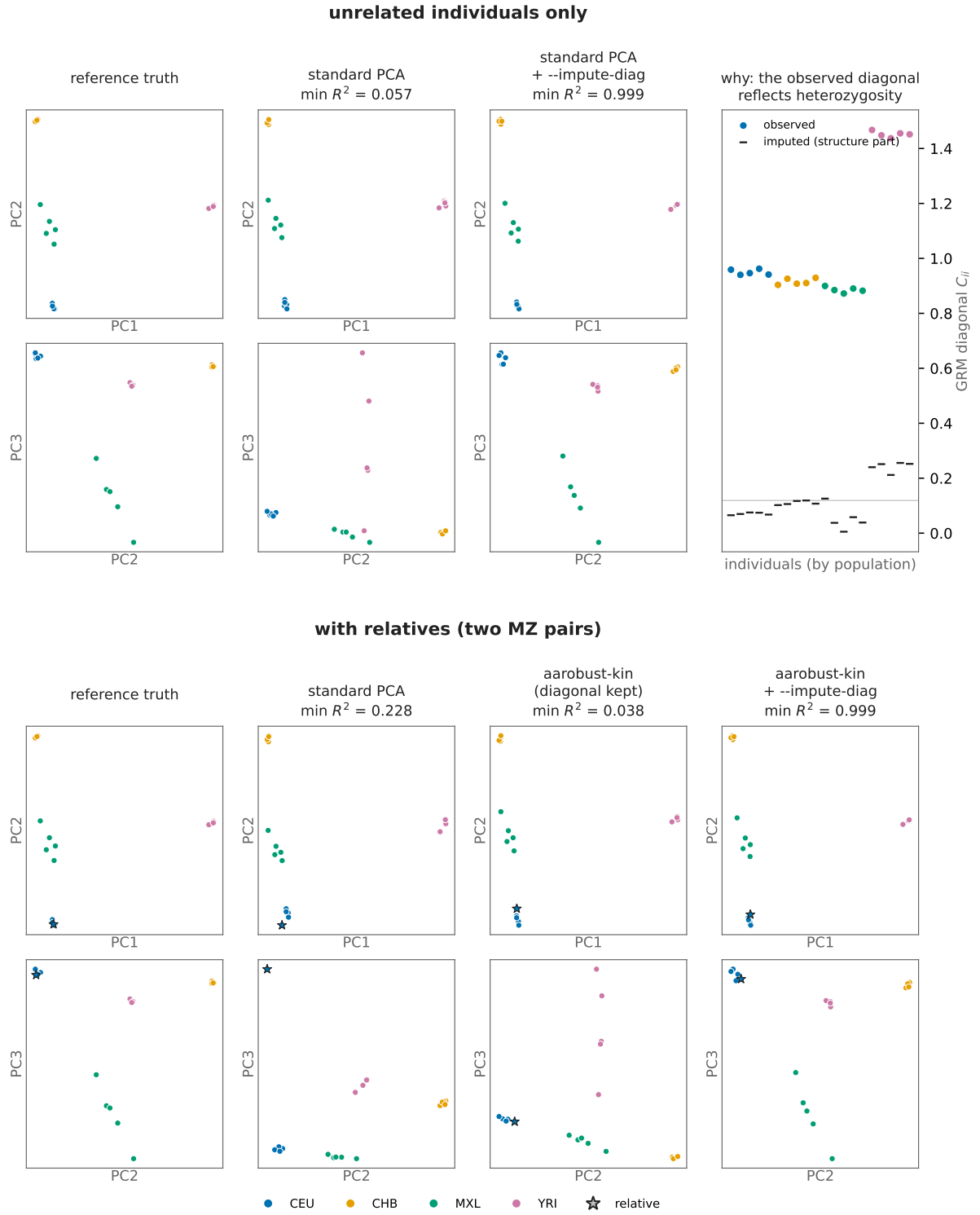
Figure 6: The small- N problem at n = 5 per population (admixTjeck2, 54k SNPs). Top: 20 unrelated individuals; the right panel shows each individual's observed GRM diagonal and its imputed structure part. Bottom: the same individuals plus two MZ twins (stars). Each method's PCs are mapped onto the reference truth by least squares on the unrelated individuals; min R^2 is the worst of the three axes.
