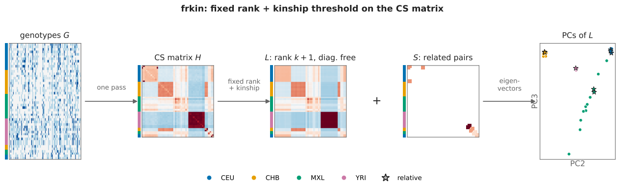
Figure 12: Graphical abstract of frkin : the detection fit of detect-white at fixed rank k + 1 ; the PCs are taken from L .
