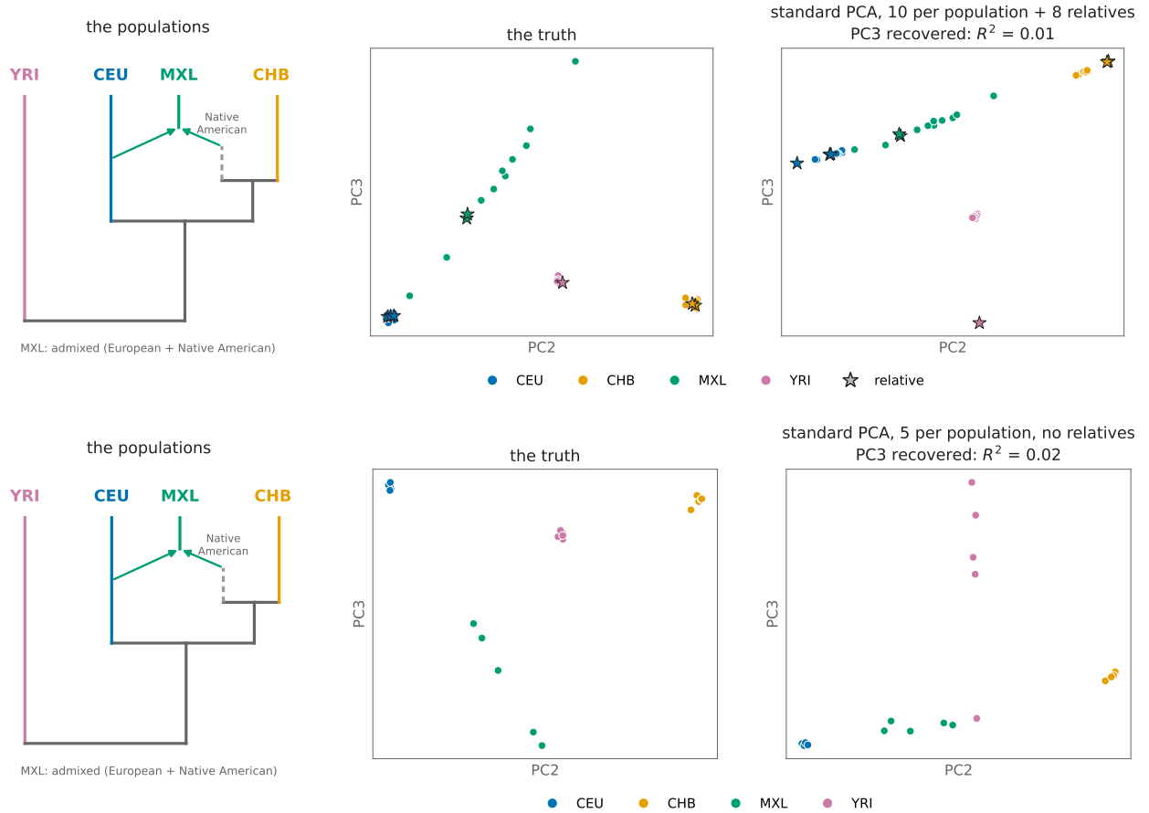
Figure 1: The problem. Left: the populations (MXL is admixed, European and Native American). Middle: the reference truth (PC2 vs PC3). Right: standard PCA mapped onto the truth by least squares on the unrelated individuals. Top: 10 unrelated individuals per population plus 8 relatives (stars); PC3 is lost ( R^2 = 0.01 ). Bottom: 5 individuals per population, no relatives; PC3 is lost as well ( R^2 = 0.02 ). admixTjeck2 genotypes, 54k SNPs; made by scripts/relatepca/slides_hook.py .
