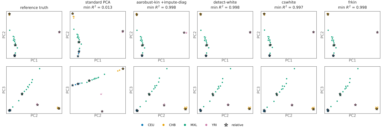
Figure 2: The example ( N = 48 , 4 populations, 8 relatives as stars). Top row: PC1 vs PC2; bottom row: PC2 vs PC3. The reference truth is a PCA of the 326 admixTjcek2 individuals not in the sample, onto which the sample is projected. Each method’s PCs are mapped onto the truth by least squares on the unrelated individuals, and \min R^2 is the worst of the three axes.
