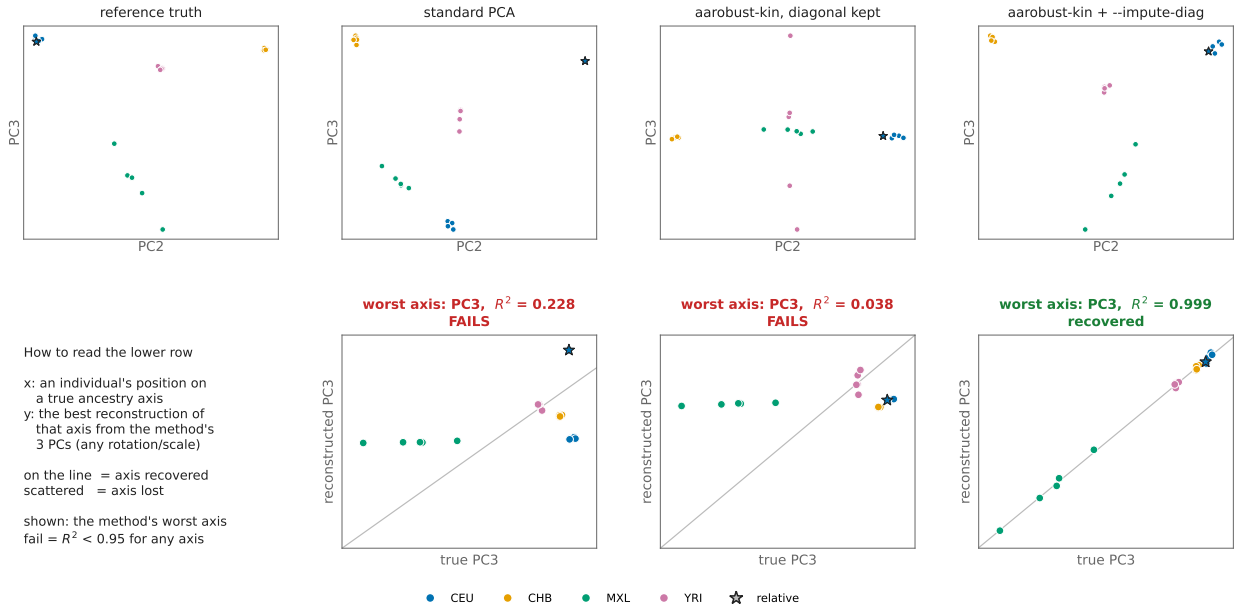
Figure 7: What “fail” means (the example of Figure 6). Upper rows: the raw PC2 and PC3 as each method returns them. Lower rows: for the method’s worst true axis, each individual’s true position ( x ) against the best reconstruction from the method’s three PCs ( y , least squares on the unrelated individuals). On the line, the axis is recovered; a run fails when R^2 < 0.95 for any of the three true axes.
