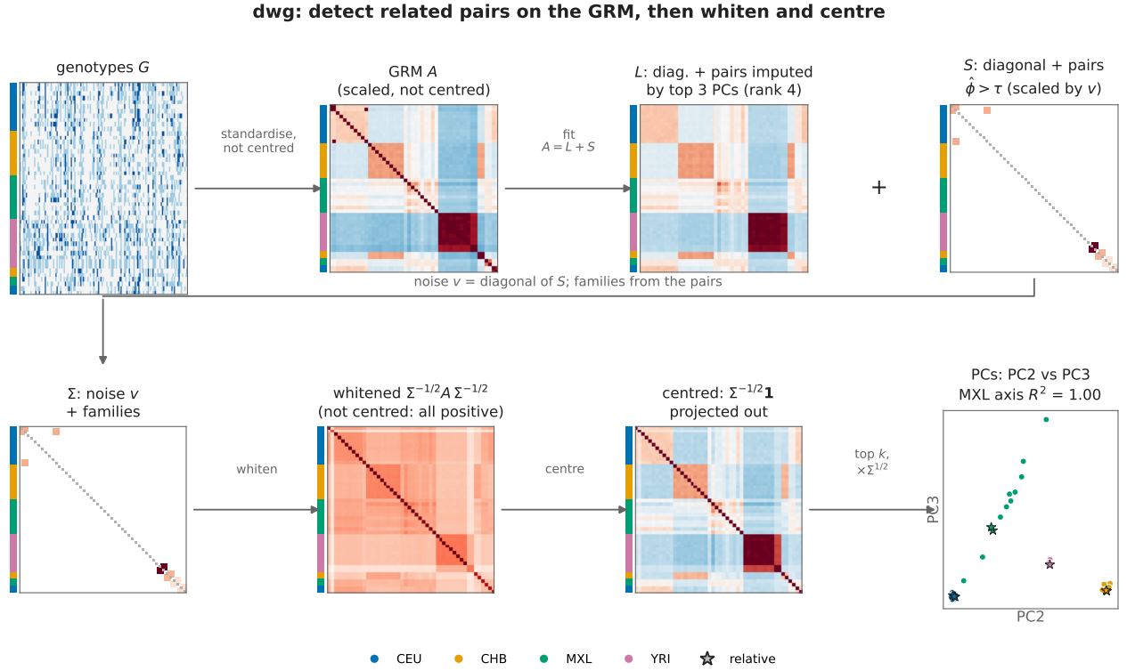
Figure 10: Graphical abstract of dwg on the example, as implemented. Top: the genotypes give the SNP-standardised but uncentred GRM A (centring would spread each person’s heterozygosity over the whole matrix). The fit A = L + S chooses rank 4 (three ancestry axes plus the mean) by the noise edge; S holds the diagonal and the six related pairs, with kinship scaled by the fitted noise v ; L = A - S has its diagonal and pair entries imputed by the top 3 PCs. Bottom: \Sigma (noise plus families) whitens A ; the whitened matrix is not centred (all positive), so \Sigma^{-1/2}\mathbf{1} , the mean direction in the whitened space, is projected out; the top k eigenvectors, mapped back by \Sigma^{1/2} , are the PCs, with PC1 the first ancestry axis. Candidates come from KING and, for relatives KING misses, from an evalAdmix screen confirmed by k_0 (not shown). A , L and the centred matrix are double-centred for display only.
