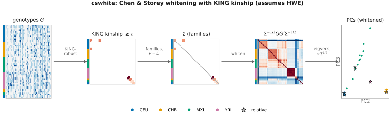
Figure 11: Graphical abstract of cswwhite . The pairs and their kinship come straight from KING-robust (or --kinship ). \Sigma uses heterozygosity D as the noise variance. The whitened Gram matrix is shown with its mean removed.
