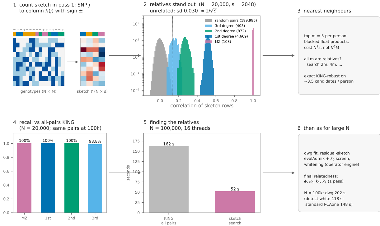
Figure 5: Very large N . The search for relatives replaces KING over all pairs. A count sketch of the standardised genotypes is built in the first pass. In it, relatives have a correlation of about 2\phi and unrelated pairs about 0 \pm 1/\sqrt{s} : the histogram shows all 6052 true pairs of the simulated N = 20,000 data against 200,000 random pairs. Each person's 5 nearest neighbours are checked with exact KING. This finds every MZ, 1st- and 2nd-degree pair, at a third of the time of KING over all pairs at N = 100,000 . The rest of the pipeline is that of large N (dwg).
