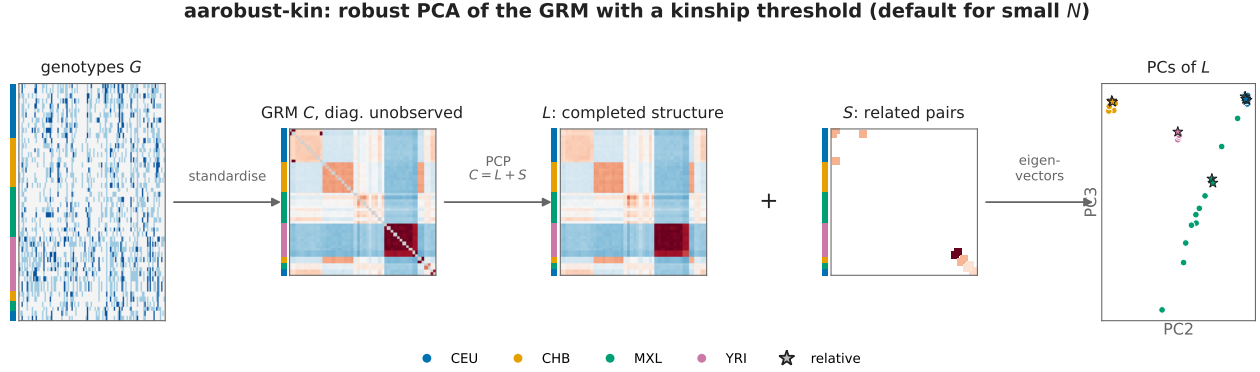
Figure 8: Graphical abstract of aarobust-kin on the example. Individuals are ordered by population; each relative is placed right after its closest kin. The GRM’s diagonal (grey) is treated as unobserved. PCP splits the GRM into L , the completed structure, and S , which holds the six related pairs and the diagonal. The PCs shown are those of L , as given with --impute-diag . Without it, they are the PCs of the GRM with the related entries replaced by L and the observed diagonal kept.
