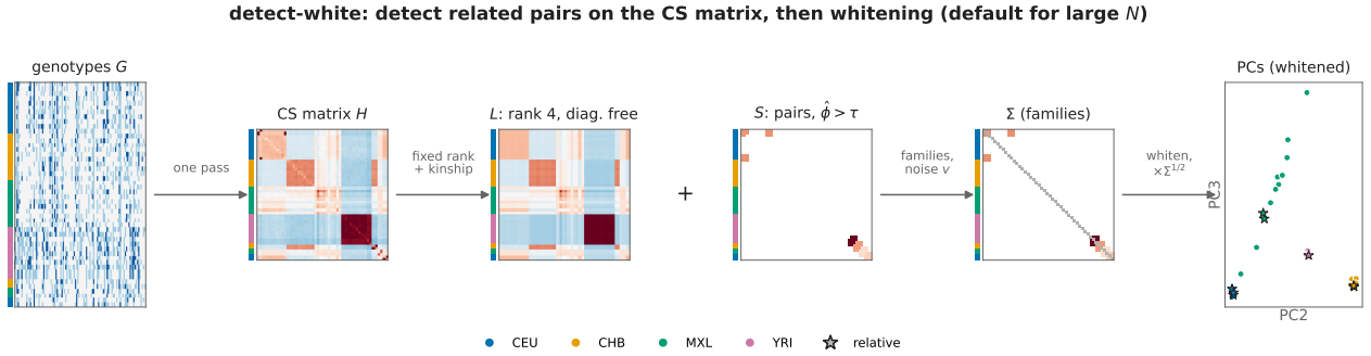
Figure 9: Graphical abstract of detect-white . The CS matrix and L are double-centred for display only (the mean component would otherwise dominate). The noise edge chose rank 4 (three ancestry axes plus the mean). S holds the detected pairs. \Sigma is block diagonal: one block per family, a scalar for everyone else.
