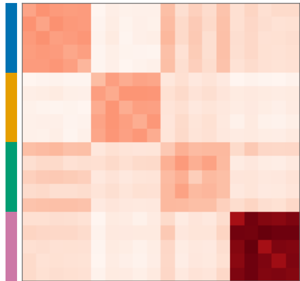
CS covariance H (not centred: all positive)
