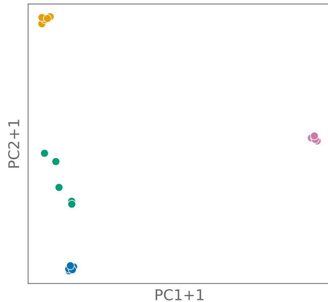
PC1+1 vs PC2+1: the ancestry
