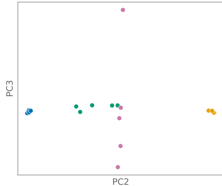
standard PCA, 5 per population, no relatives PC3 recovered: R^2 = 0.02
