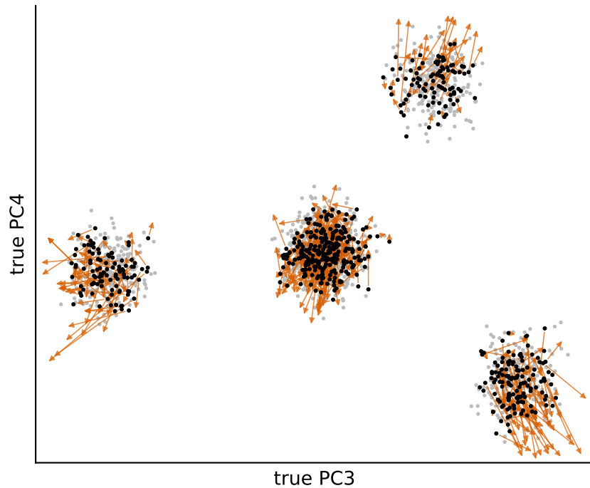
standard PCA: relatives' error 0.45
