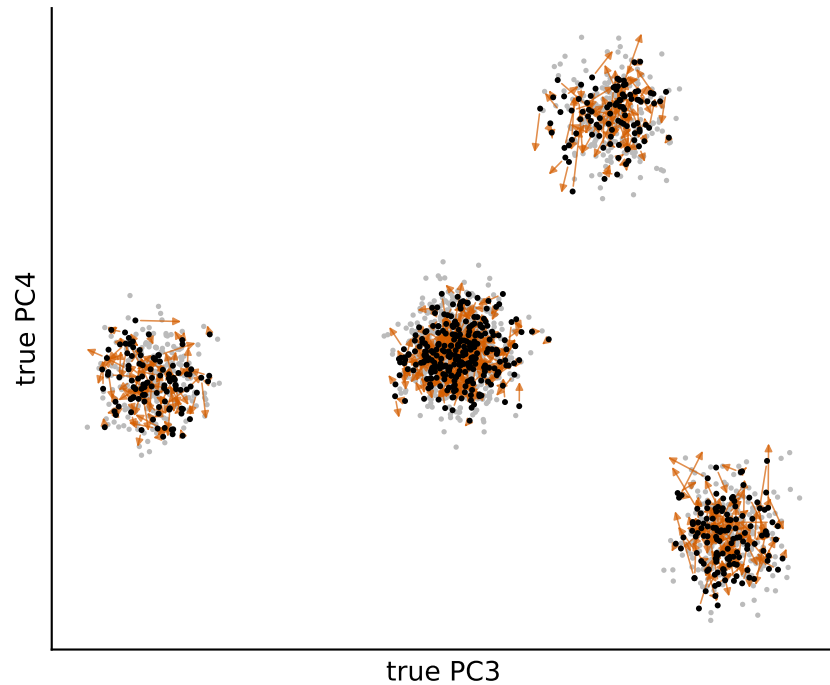
robust (dwg): relatives' error 0.11
