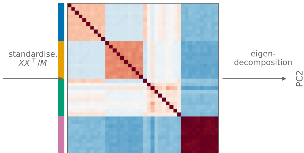
covariance between individuals (GRM)
