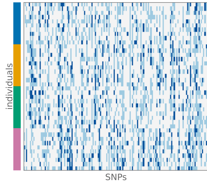
genotypes (0/1/2), 150 of 53k SNPs
