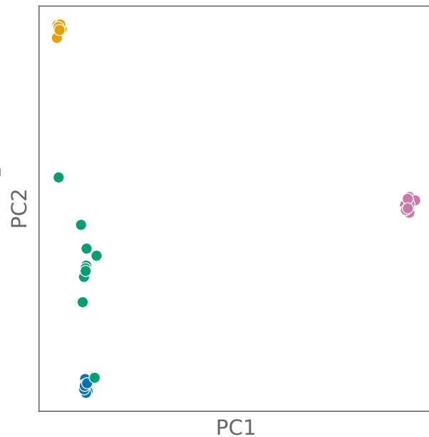
PCs: top eigenvectors
