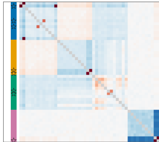
GRM minus top 2 PCs (diagonal hidden)
