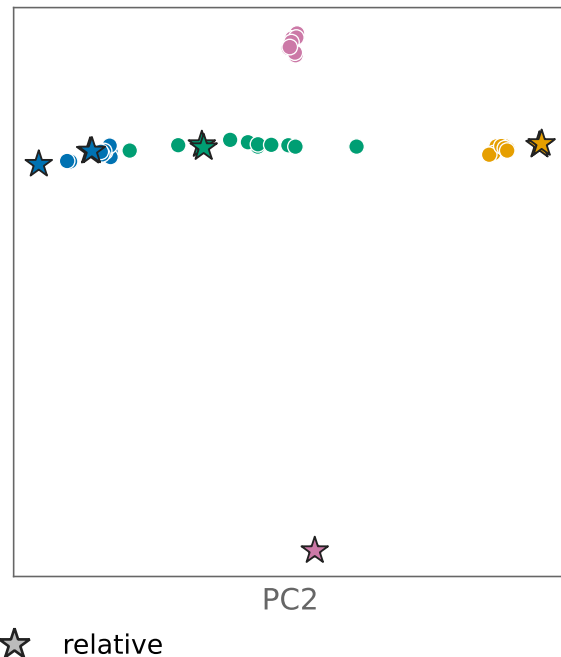
so PC3 follows the relatives
