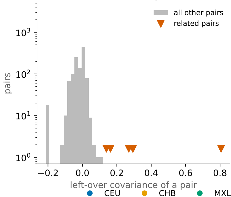
what is left: the related pairs stand out
