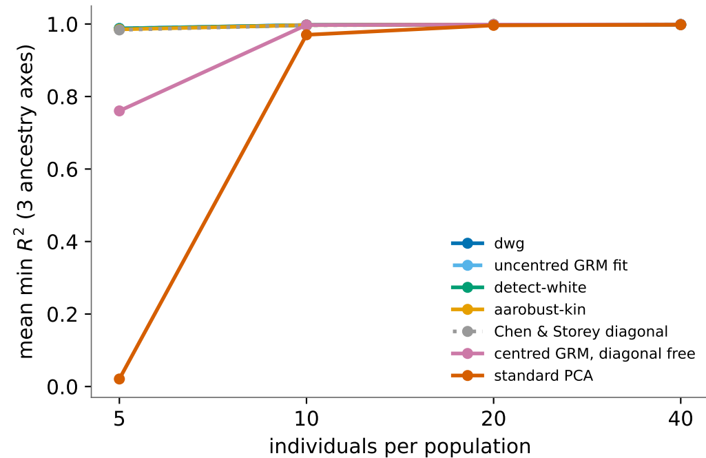
accuracy, no relatives
