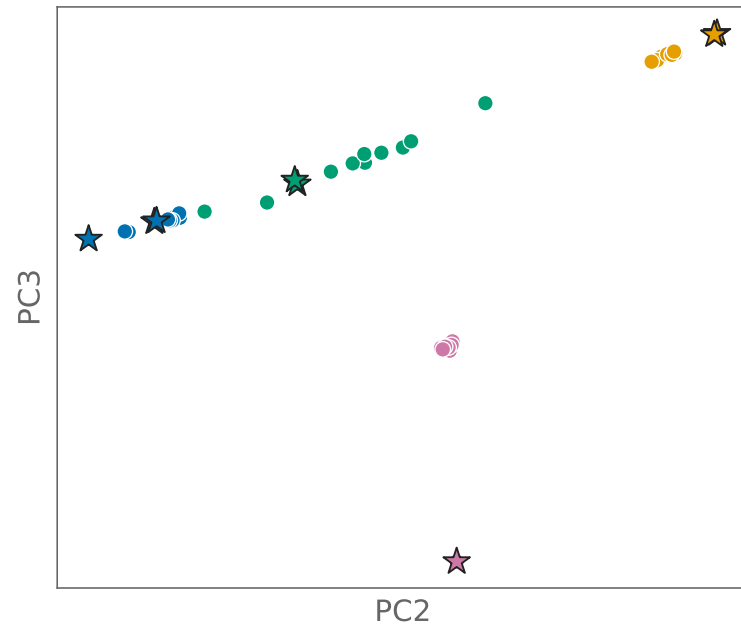
standard PCA, 10 per population + 8 relatives PC3 recovered: R^2 = 0.01
