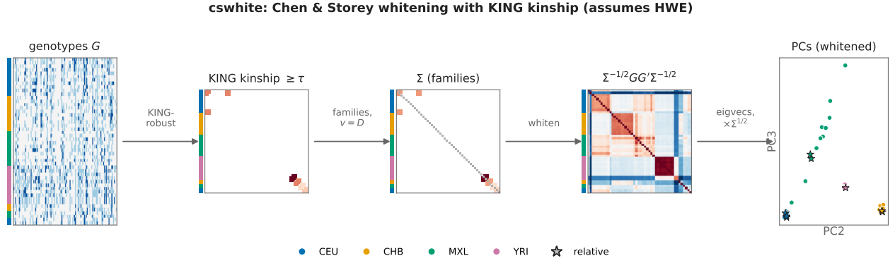
Figure 10: Graphical abstract of cswwhite . The pairs and their kinship come straight from KING-robust (or --kinship ). \Sigma uses heterozygosity D as the noise variance. The whitened Gram matrix is shown with its mean removed.
