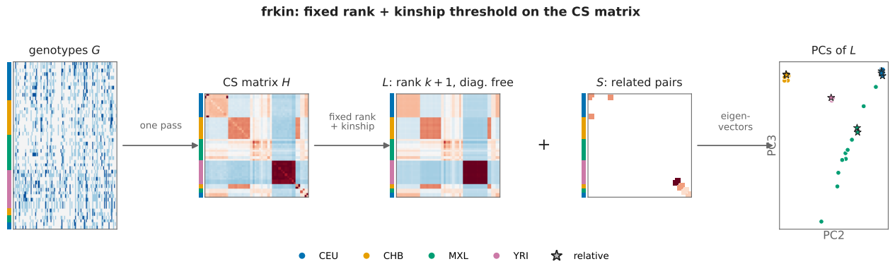
Figure 11: Graphical abstract of frkin : the detection fit of detect-white at fixed rank k + 1 ; the PCs are taken from L .
