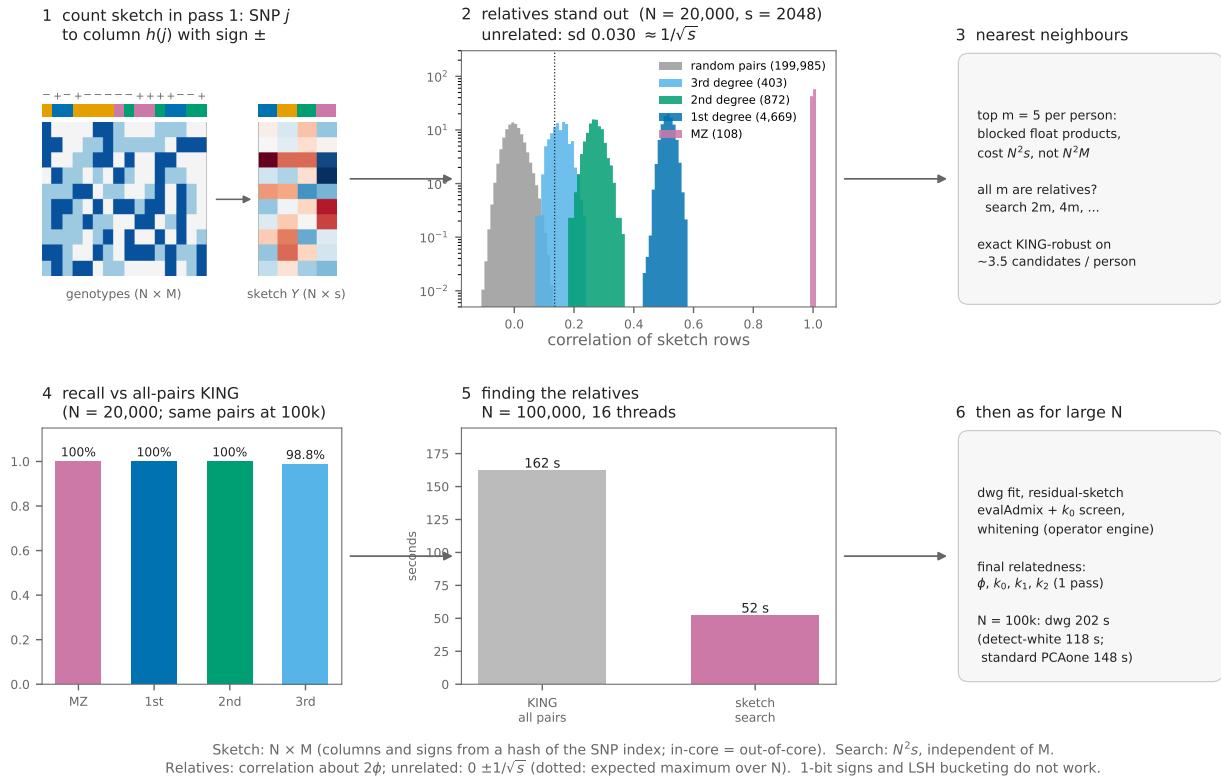
Figure 4: Very large N . The search for relatives replaces KING over all pairs. A count sketch of the standardised genotypes is built in the first pass. In it, relatives have a correlation of about 2\phi and unrelated pairs about 0 \pm 1/\sqrt{s} : the histogram shows all 6052 true pairs of the simulated N = 20,000 data against 200,000 random pairs. Each person's 5 nearest neighbours are checked with exact KING. This finds every MZ, 1st- and 2nd-degree pair, at a third of the time of KING over all pairs at N = 100,000 . The rest of the pipeline is that of large N (dwg).
