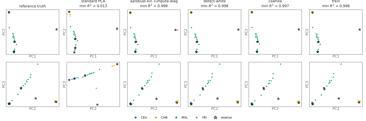
Figure 1: The example ( N = 48 , 4 populations, 8 relatives as stars). Top row: PC1 vs PC2; bottom row: PC2 vs PC3. The reference truth is a PCA of the 326 admixTjcek2 individuals not in the sample, onto which the sample is projected. Each method’s PCs are mapped onto the truth by least squares on the unrelated individuals, and min R^2 is the worst of the three axes.
