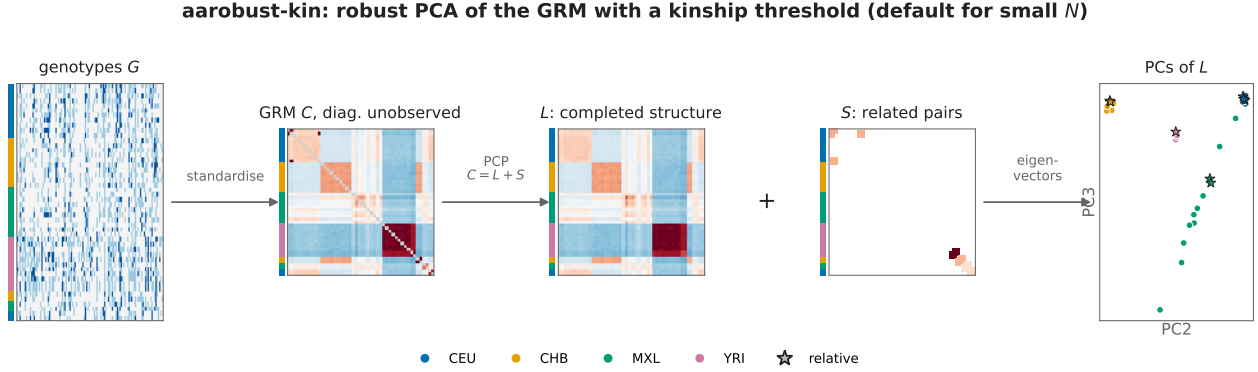
Figure 7: Graphical abstract of aarobust-kin on the example. Individuals are ordered by population; each relative is placed right after its closest kin. The GRM’s diagonal (grey) is treated as unobserved. PCP splits the GRM into L , the completed structure, and S , which holds the six related pairs and the diagonal. The PCs shown are those of L , as given with --impute-diag . Without it, they are the PCs of the GRM with the related entries replaced by L and the observed diagonal kept.
