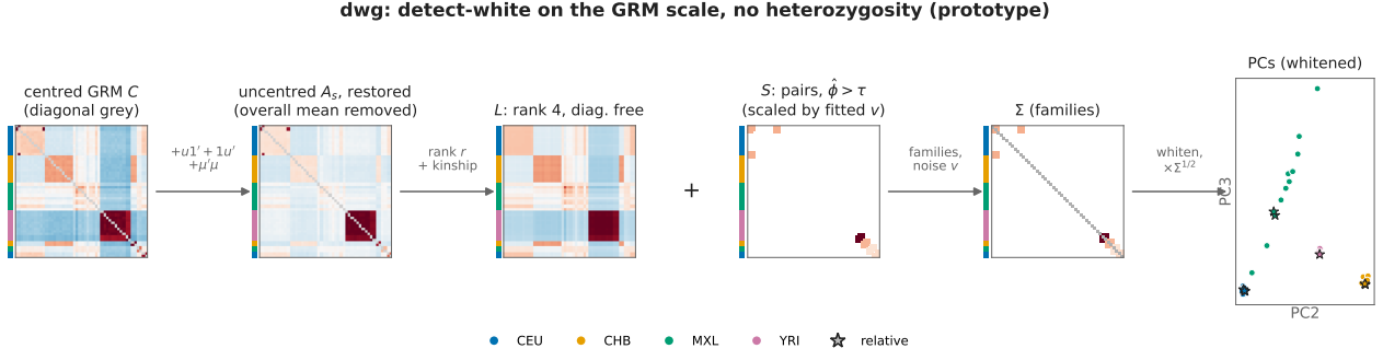
Figure 9: Graphical abstract of dwg on the example. The centred GRM (what centred data give) is turned back into the uncentred, SNP-standardised Gram A_s with the allele frequencies and one number per individual ( u = X_c \mu / M ). In C the YRI rows are pulled negative by their high heterozygosity, spread over the off-diagonal entries by the centring; in A_s this sits in the mean component instead. The fit chooses rank 4 (three ancestry axes plus the mean) and finds the six related pairs, with kinship scaled by the fitted noise v rather than heterozygosity. Whitening with the family covariance \Sigma gives the PCs. Candidates come from KING and, for relatives KING misses, from an evalAdmix screen confirmed by k_0 (not shown). Matrices shown without the diagonal (grey) and, for A_s , with the overall mean removed; L is double-centred for display only.
