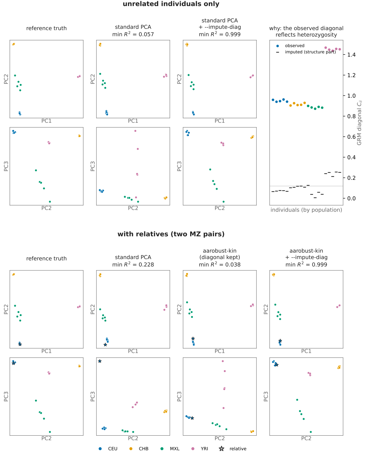
Figure 5: The small- N problem at n = 5 per population (admixTjeck2, 54k SNPs). Top: 20 unrelated individuals; the right panel shows each individual's observed GRM diagonal and its imputed structure part. Bottom: the same individuals plus two MZ twins (stars). Each method's PCs are mapped onto the reference truth by least squares on the unrelated individuals; min R^2 is the worst of the three axes.
