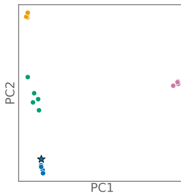
aarobust-kin (diagonal kept) min R^2 = 0.038
