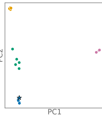
aarobust-kin + --impute-diag min R^2 = 0.999
