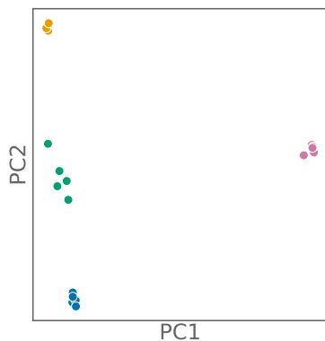
standard PCA min R^2 = 0.057
