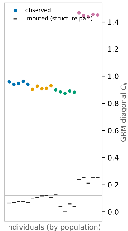
why: the observed diagonal reflects heterozygosity
