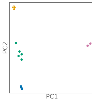
standard PCA + --impute-diag min R^2 = 0.999
