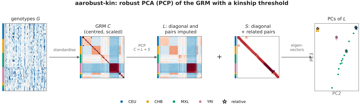
Figure 8: Graphical abstract of aarobust-kin on the example. Individuals are ordered by population; each relative is placed right after its closest kin. The GRM’s diagonal (grey) is treated as unobserved. PCP splits the GRM into L , the completed structure, and S , which holds the six related pairs and the diagonal. The PCs shown are those of L , as given with --impute-diag . Without it, they are the PCs of the GRM with the related entries replaced by L and the observed diagonal kept.
