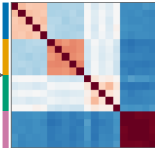
standard GRM (centred, scaled)
