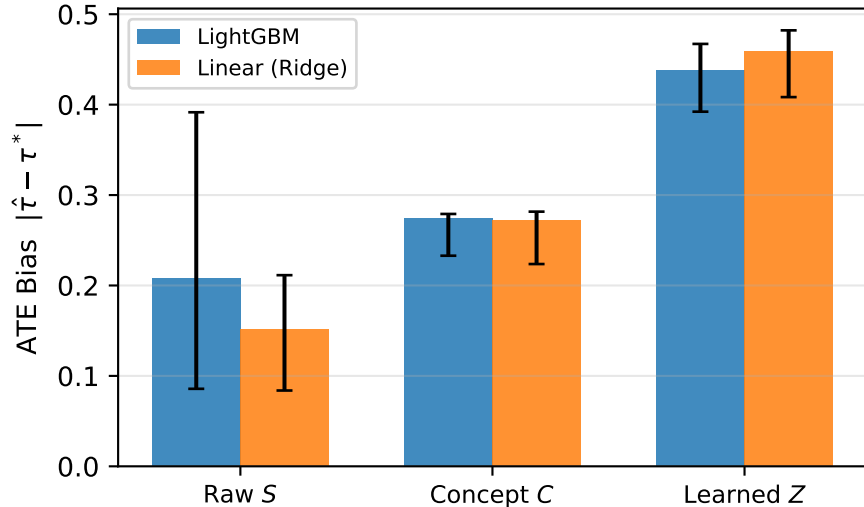
(b) Nuisance-swap robustness at N = 1,000
