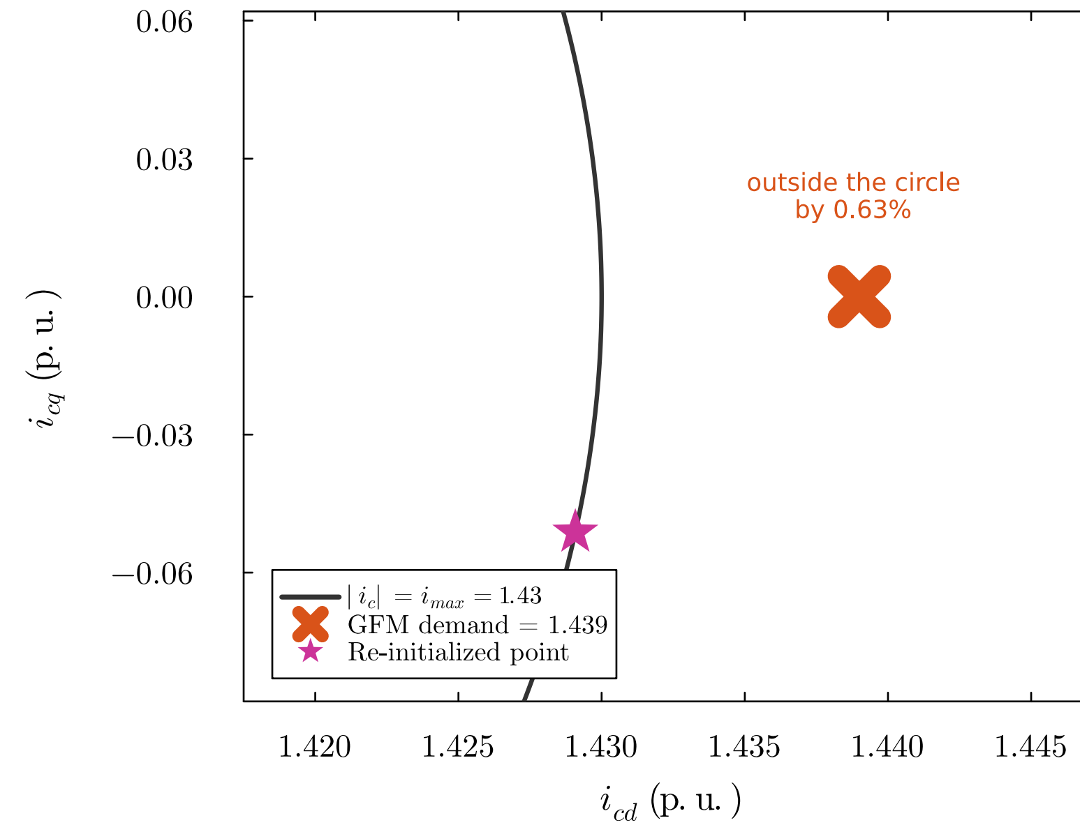
(e) Converter current magnitude
