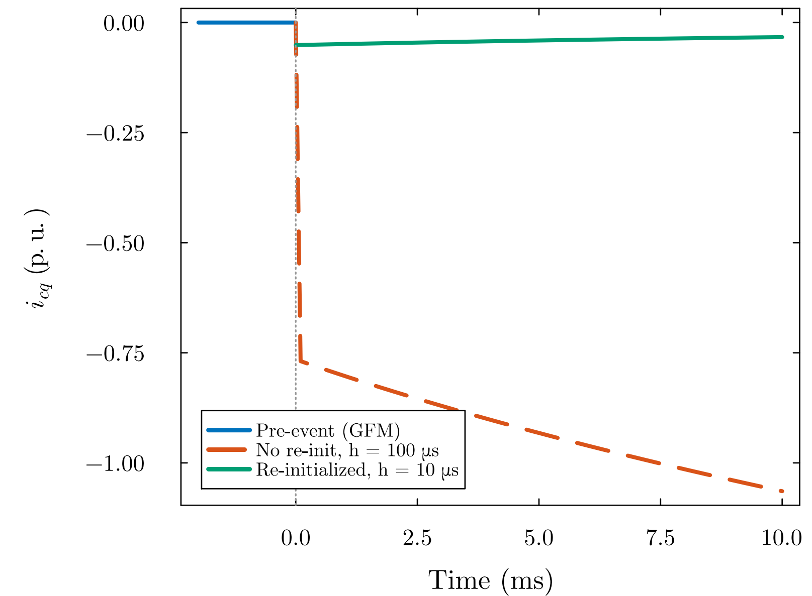
(f) Converter q-axis current
